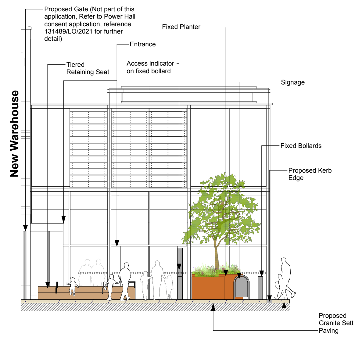
4 Proposed Section Elevation B-B Scale: 1:100
