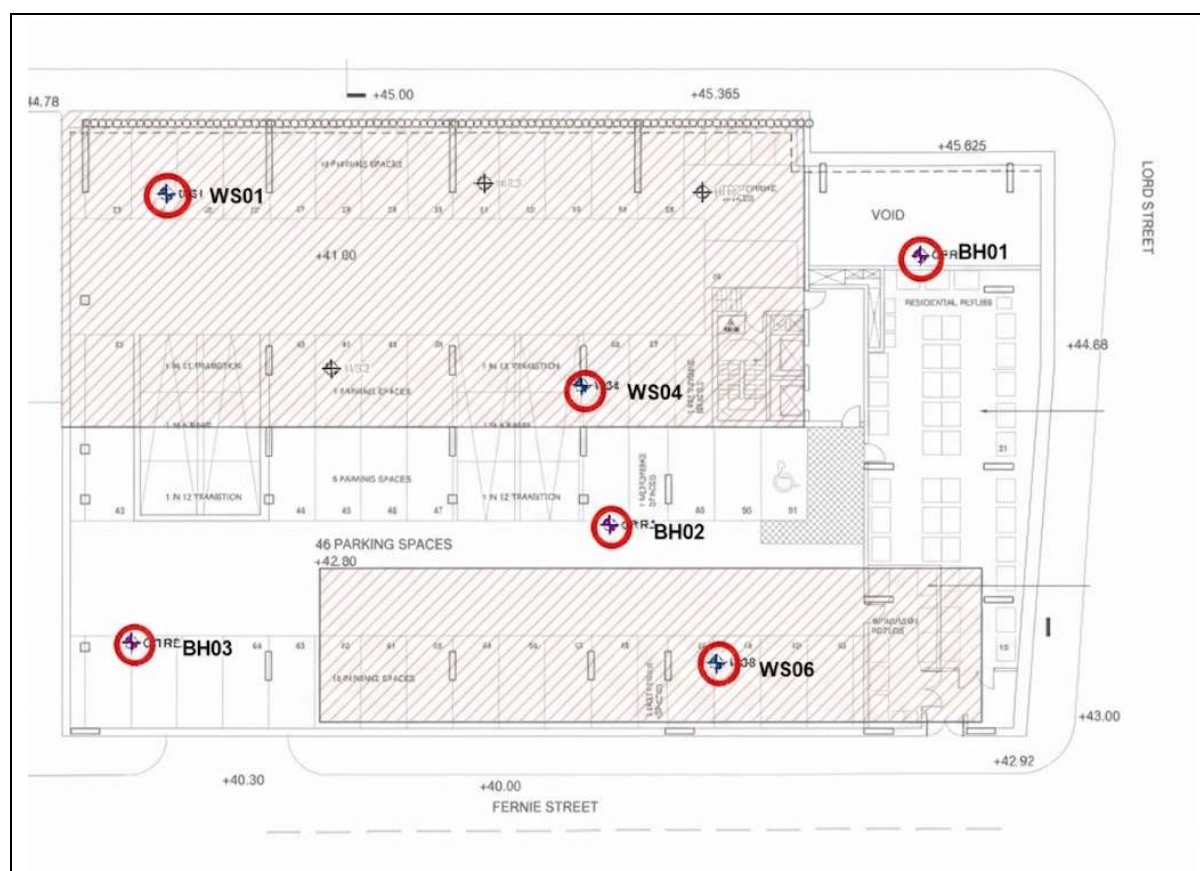
Figure 2 Previous Exploratory Hole Location Plan (Enzygo, 2019)
