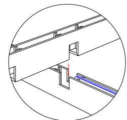
PANEL INTERLOCKING DETAIL
