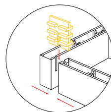
BEAM CONNECTOR DETAIL
