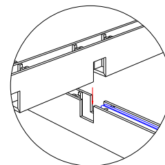
PANEL INTERLOCKING DETAIL
