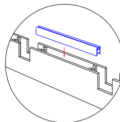
TECH RAIL FIXING DETAIL
