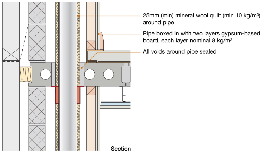
Figure 5-8: E-FC-12 typical detail for service pipes through separating floor
