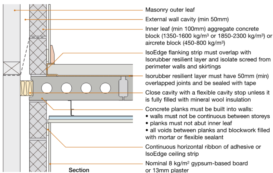
Figure 5-6: E-FC-12 External (flanking) wall junction)
