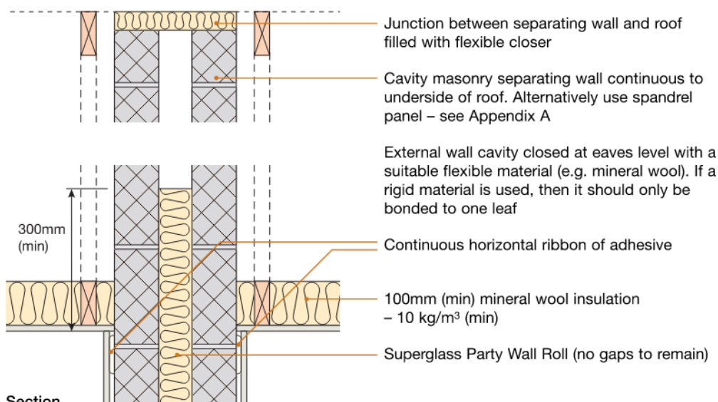
Figure 5-3: E-WM-27 roof junction – pitched roof without room-in-roof
