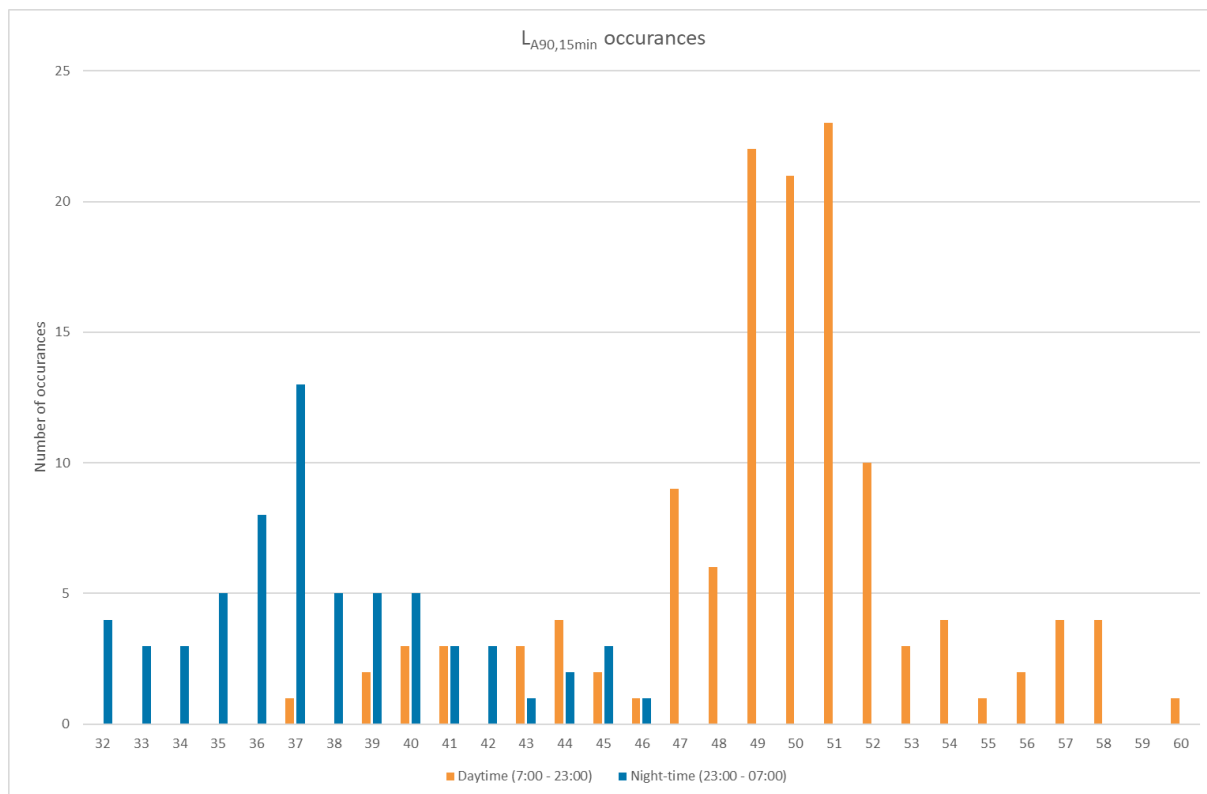
Figure 6-1: L_{A90,15min} histogram, orange = Daytime (07:00-23:00), blue = Night-time (23:00-07:00)
