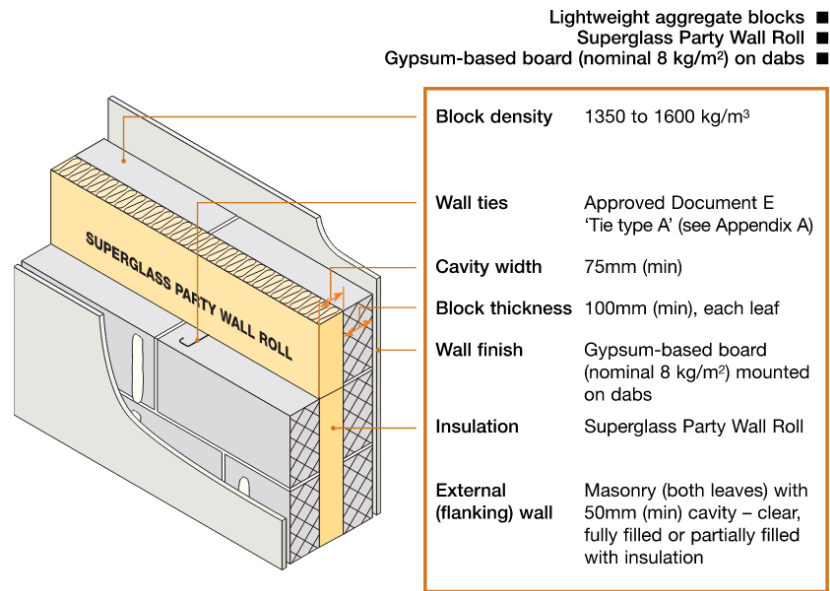
Figure 5-1: Robust Detail E-WM-27
