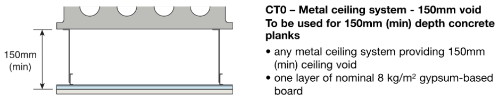
Figure 5-5: Ceiling CT0 with minimum 150 mm ceiling void
