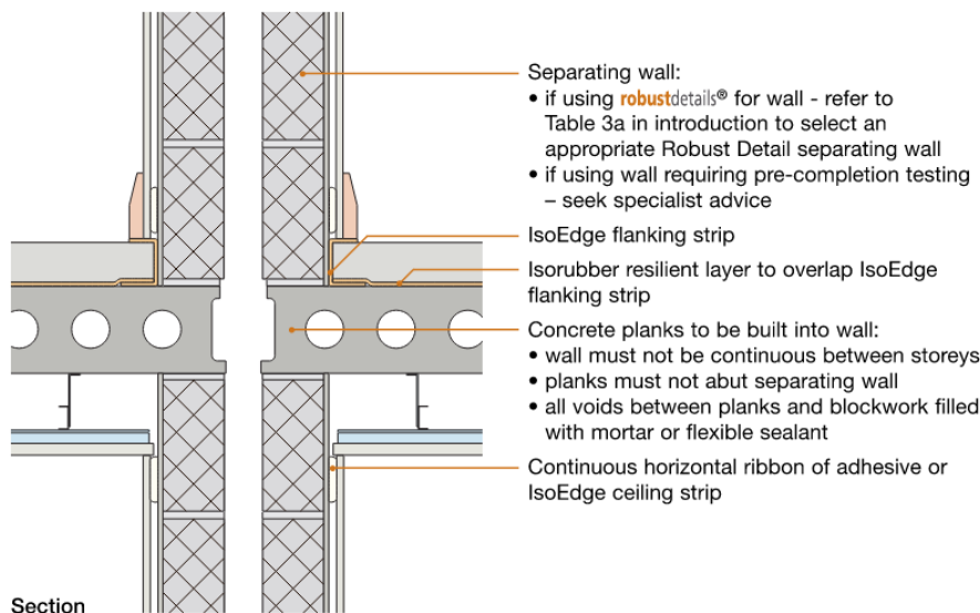
Figure 5-7: E-FC-12 Separating wall junction
