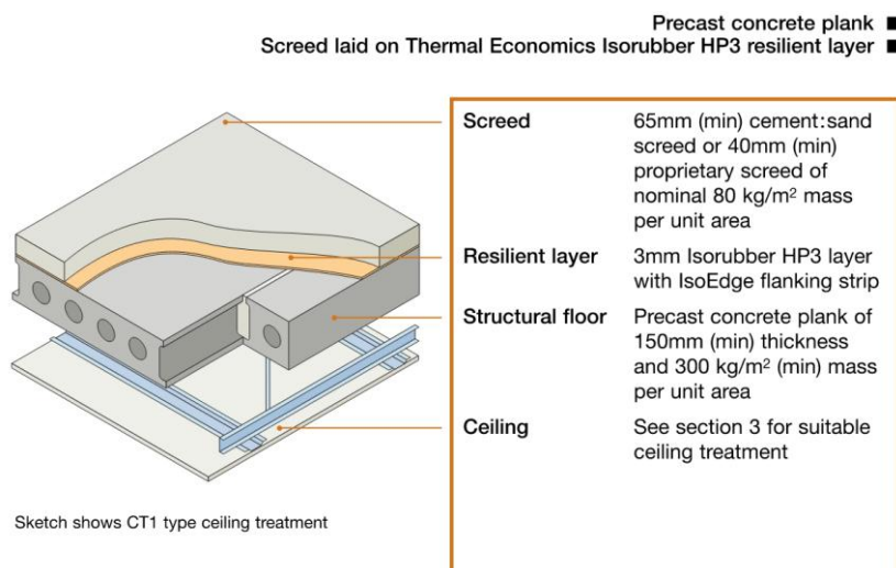
Figure 5-4: Robust Detail E-FC-12
