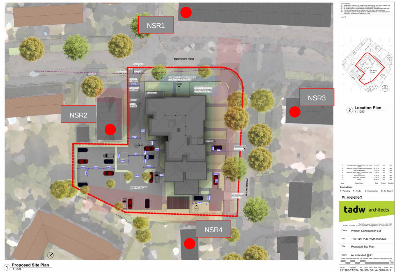
Figure 6-2: Proposed site plan (drawing 251360-TADW- 00- XX- DR- A- 0010- P- 7)
