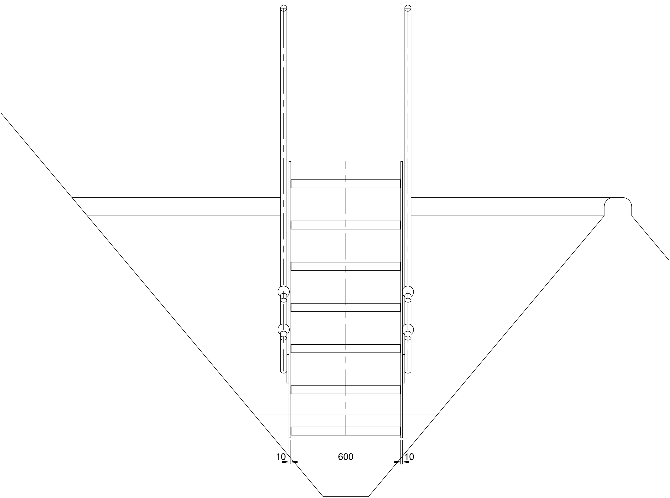
VIEW ON B - B
