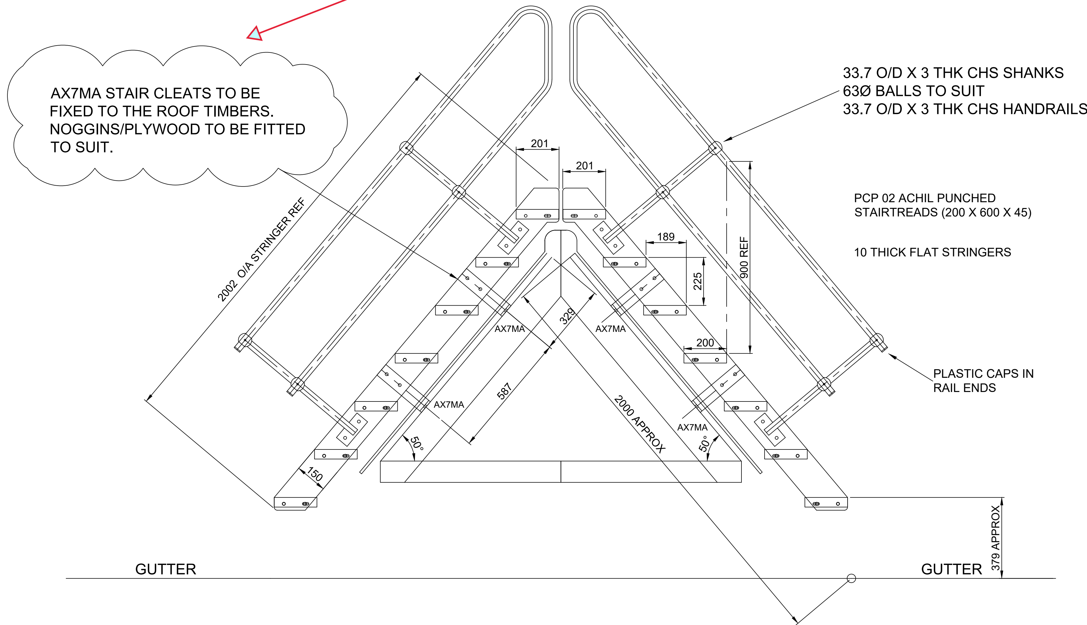
VIEW ON A - A
