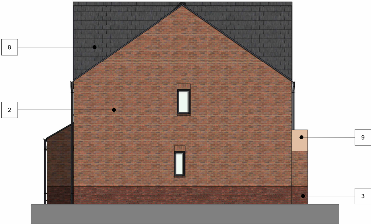
Left Elevation 1 : 100
