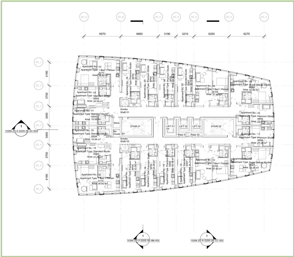
Figure 2.4 – Typical Floor Level Block D
