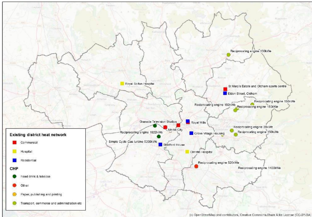
Figure 5. Existing heat networks and CHP
