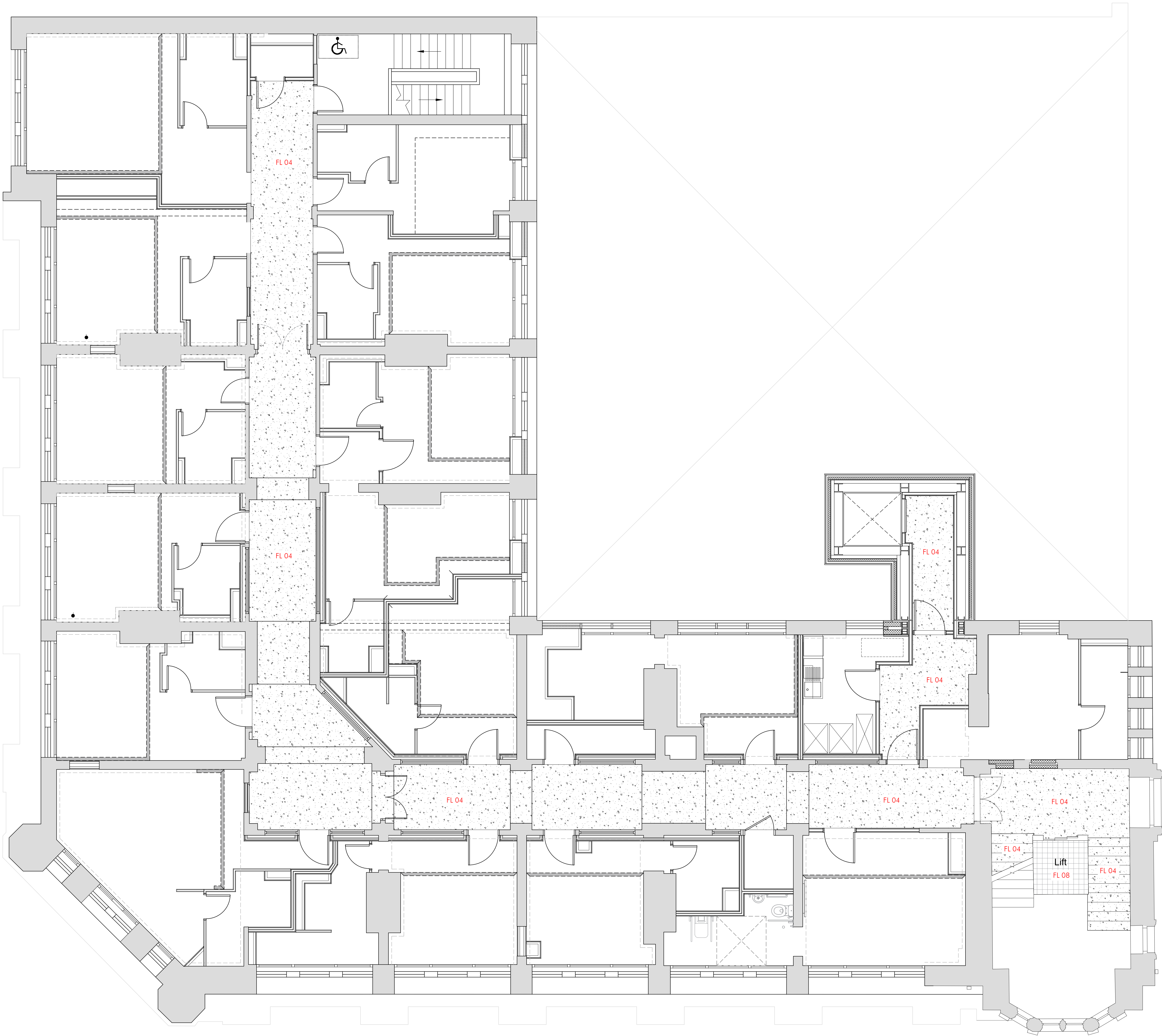
PROPOSED THIRD FLOOR LAYOUT SCALE 1:50 IN METRES
