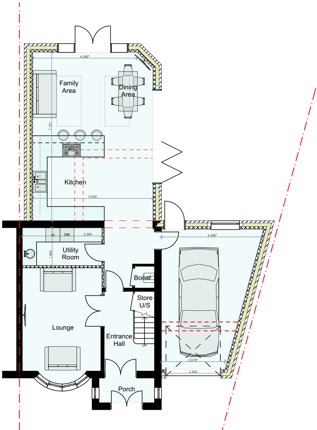
PROPOSED GA GROUND FLOOR PLAN
