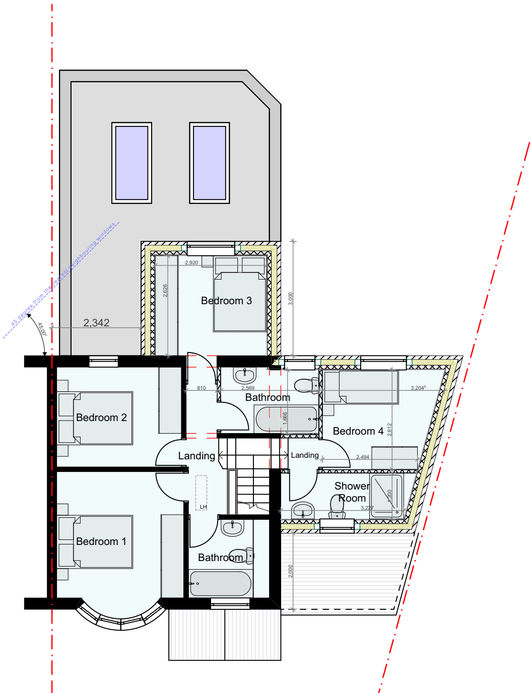
PROPOSED GA FIRST FLOOR PLAN
