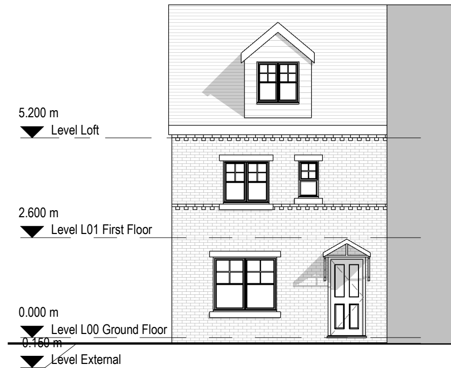
1 Existing South Elevation 1 : 100
