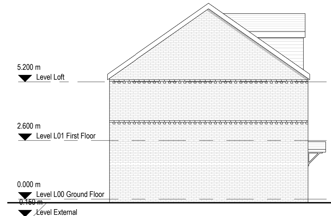
4 Existing West Elevation 1 : 100
