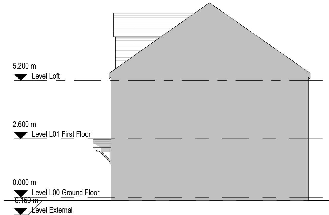
2 Existing East Elevation 1 : 100
