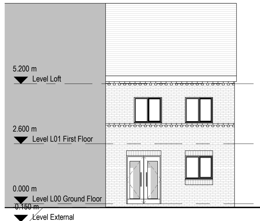
3 Existing North Elevation 1 : 100
