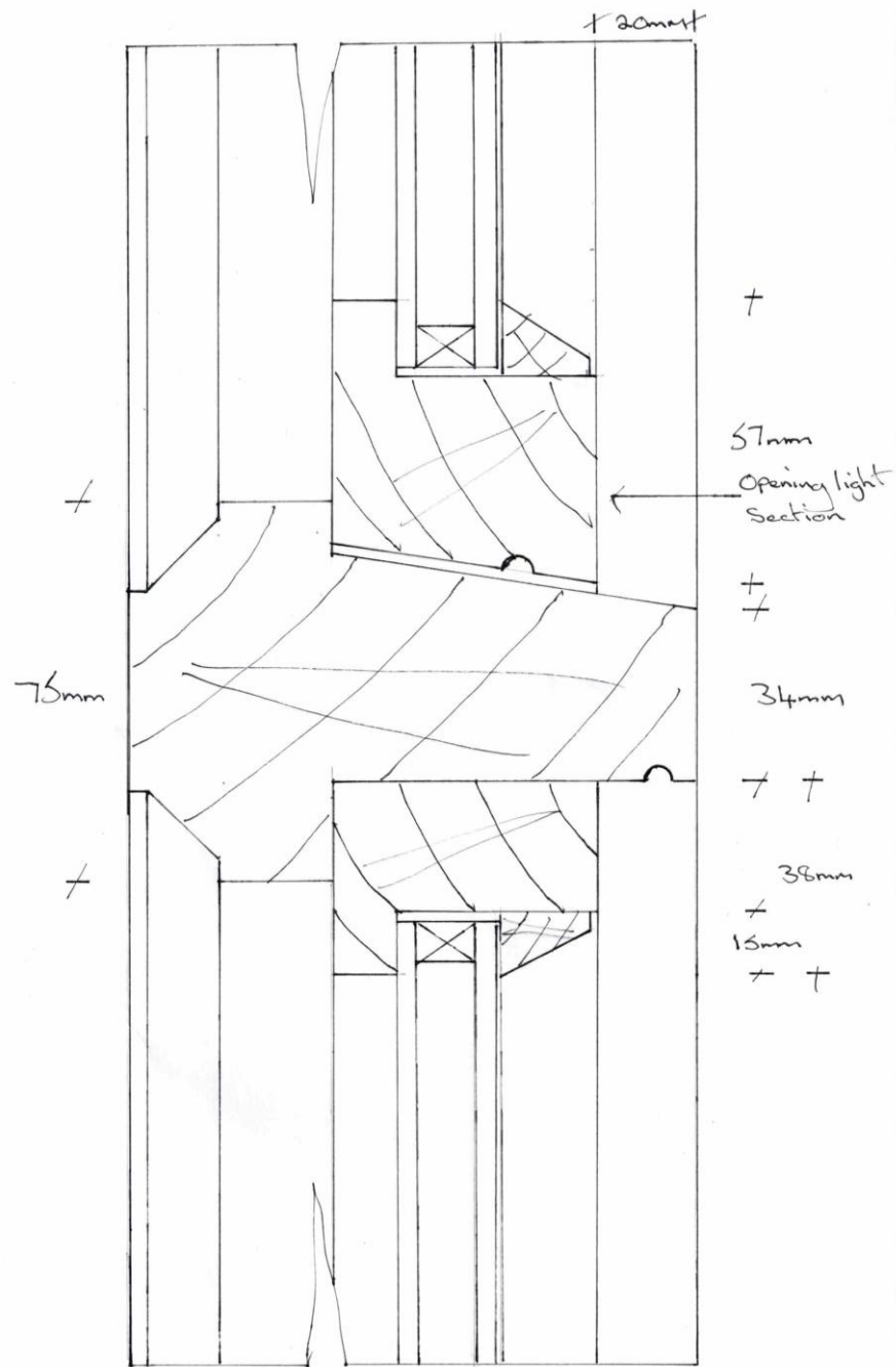
Transom detail with opening light
