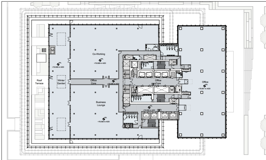
Proposed External Terrace 10518-SHA-Z1-A-B5D8-G200-PL-07-001 P01 c/o Simpson Haugh
