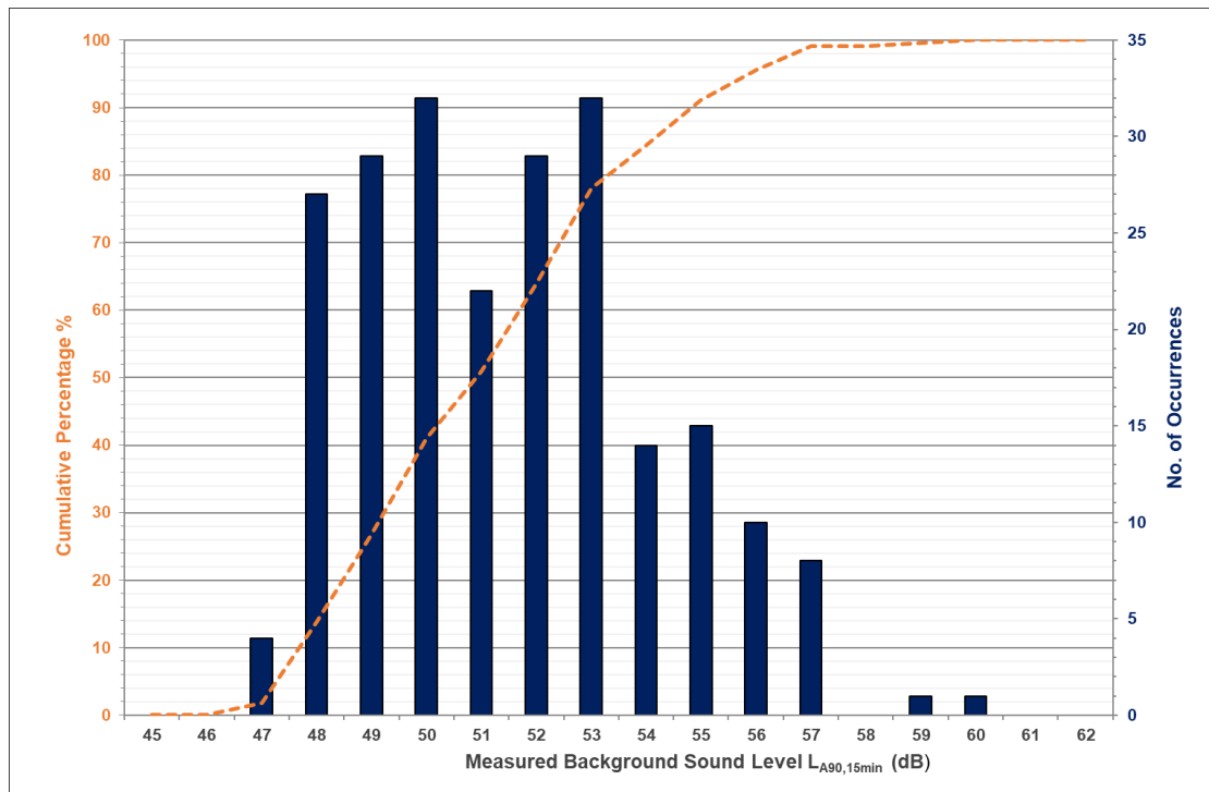
Histogram Plot of Measured Night-time Background Noise Levels – Position 5
