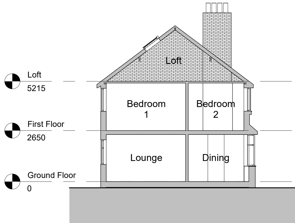
Exist. Section A
