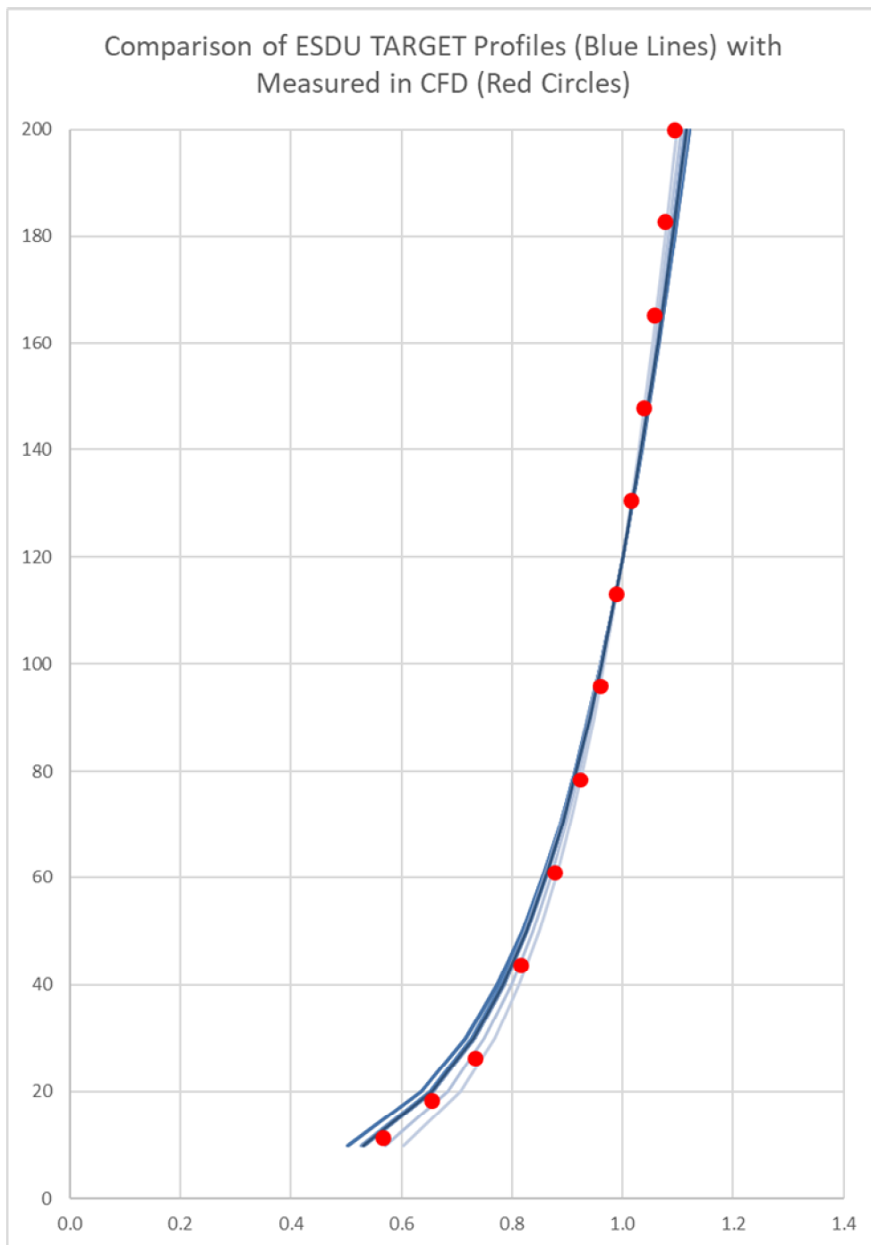
Figure 2 Wind Profile (Velocity) for Central Manchester
