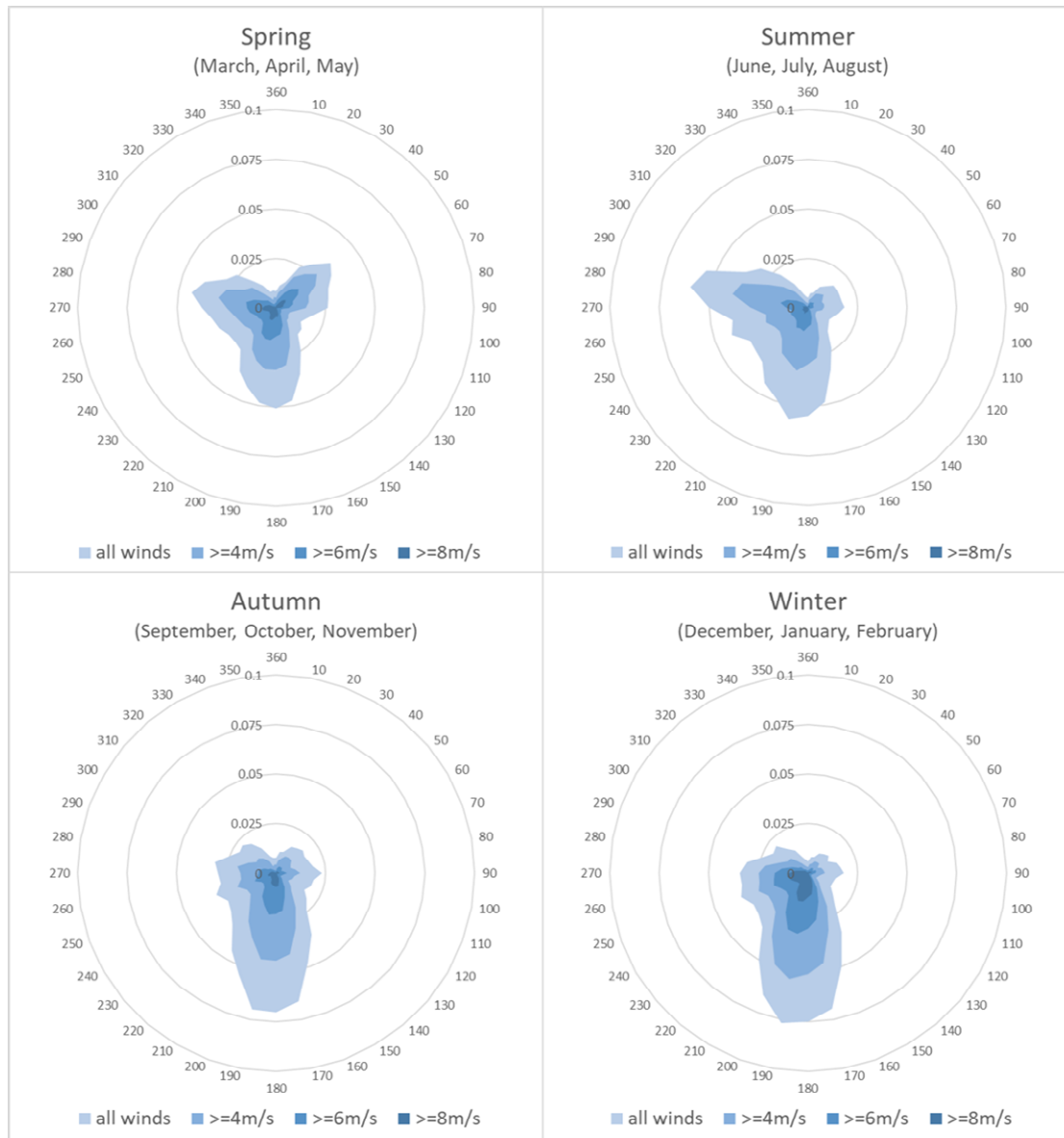
Figure 1 Seasonal Wind Roses for Manchester International Airport
