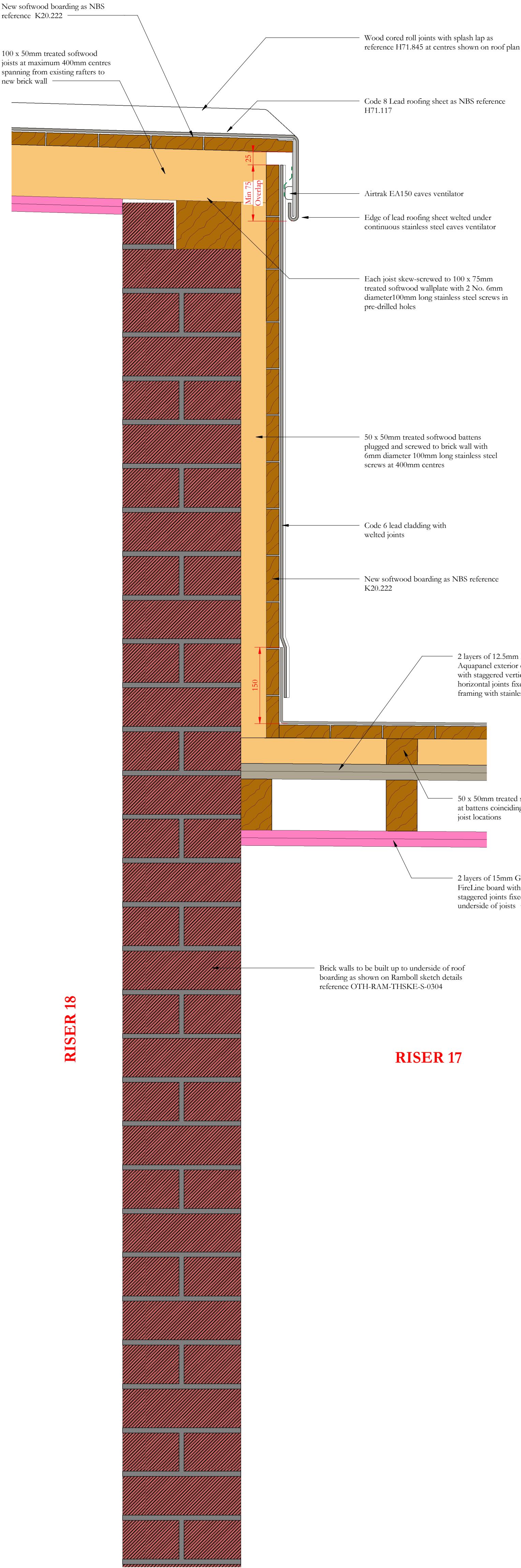
Section A-A through extended brick wall between risers 17 and 18 Scale 1:50
