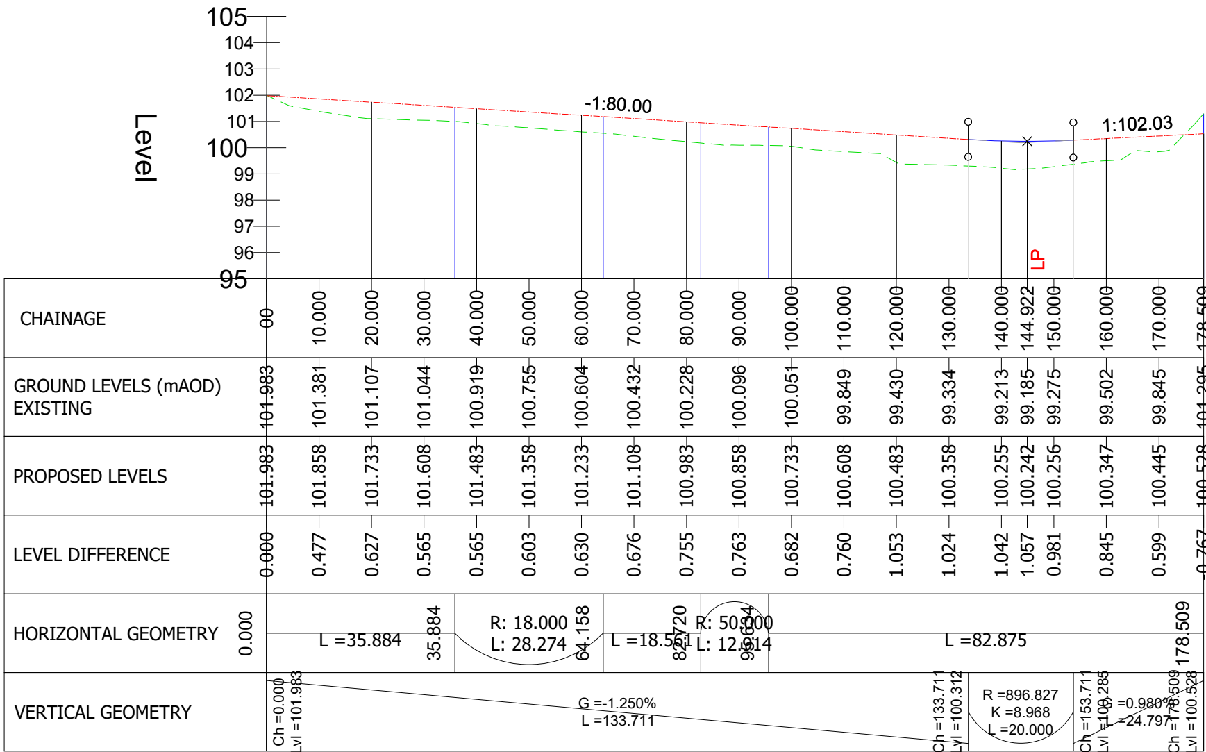
ROAD C - LONGSECTION SCALE: H 1:500,V 1:100. DATUM: 95.000
