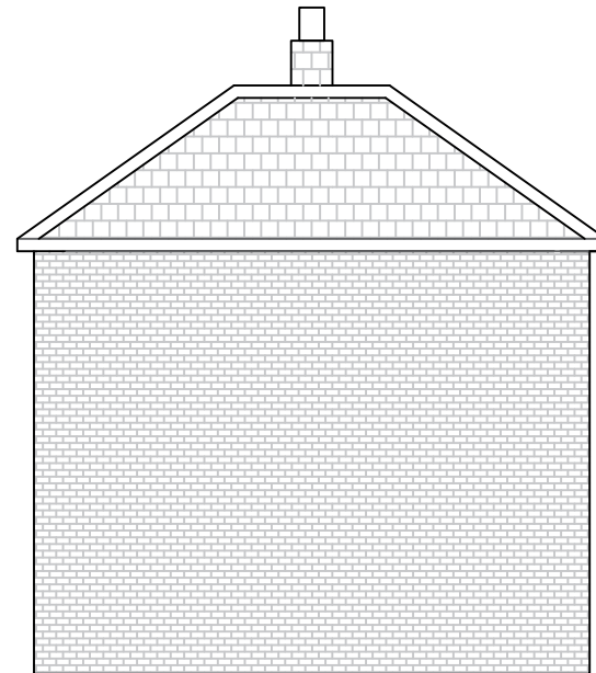
Proposed LHS Elevation
