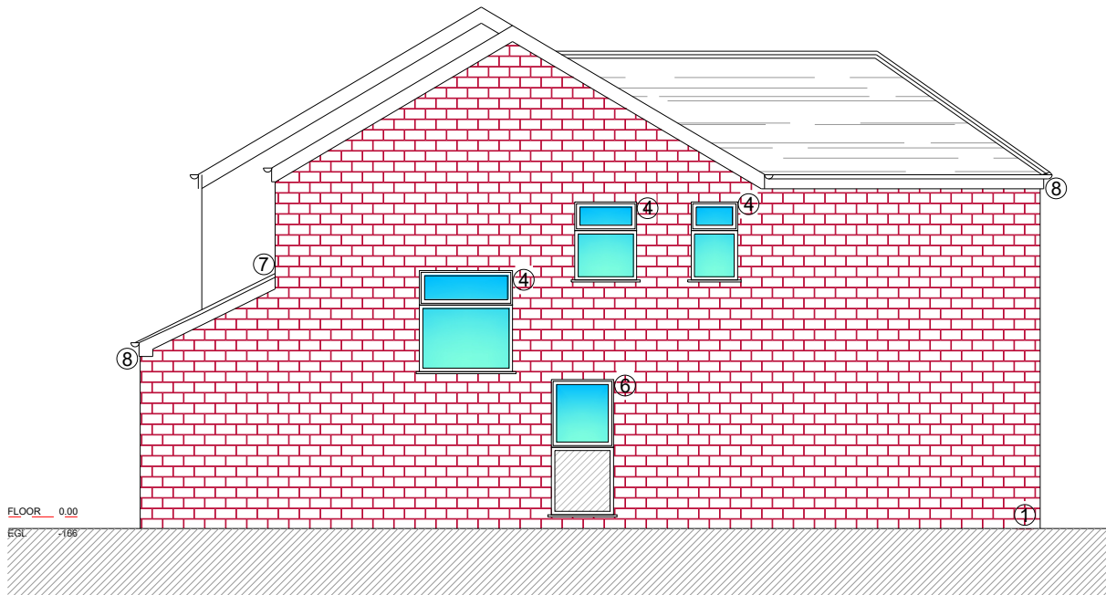
SIDE ELEVATION
