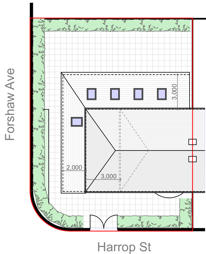
PROPOSED GA SITE PLAN
