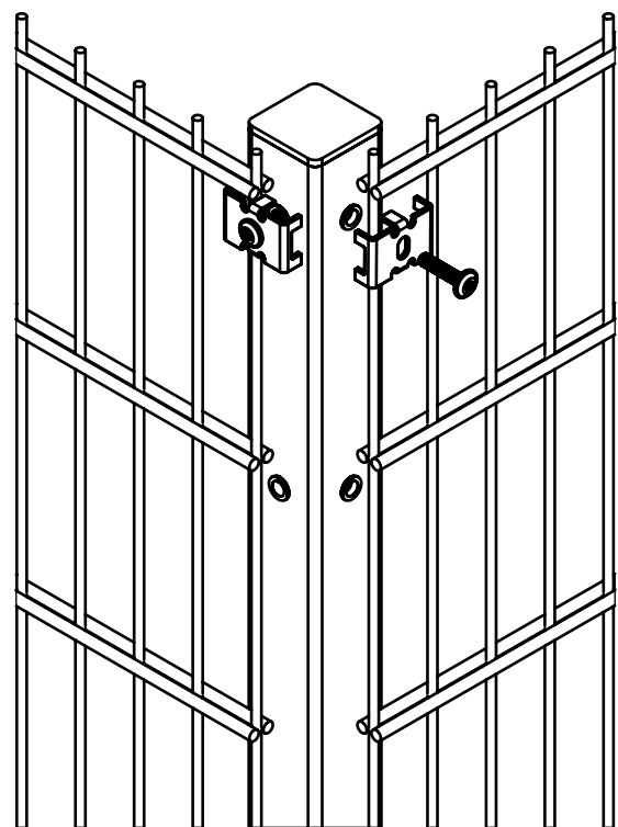
DETAIL ASSEMBLY CORNER POST
