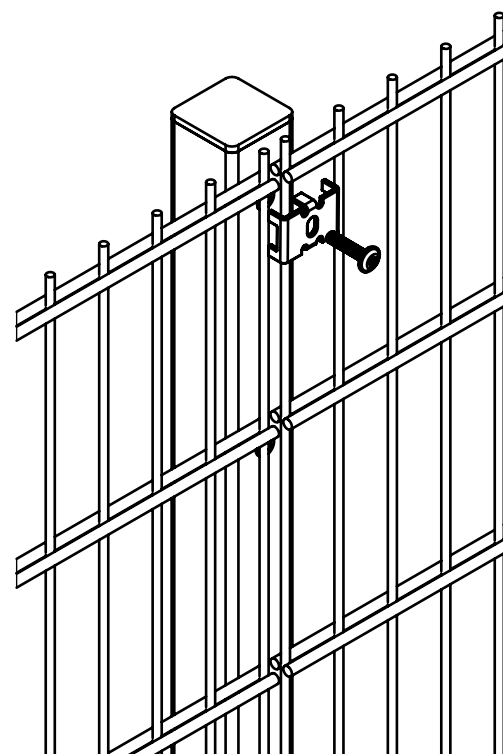
DETAIL ASSEMBLY INTERMEDIATE POST
