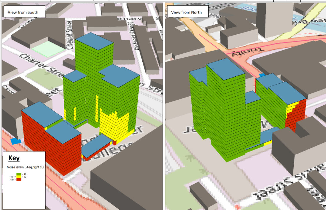
Figure 1.1 - Boddingtons ADO Risk Assessment Night-time LAeq,T Noise Levels. Cundall (1032195 MEMO AS-001)
