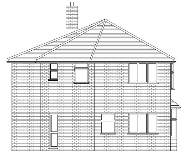
PROPOSED LEFT SIDE ELEVATION 1:100
