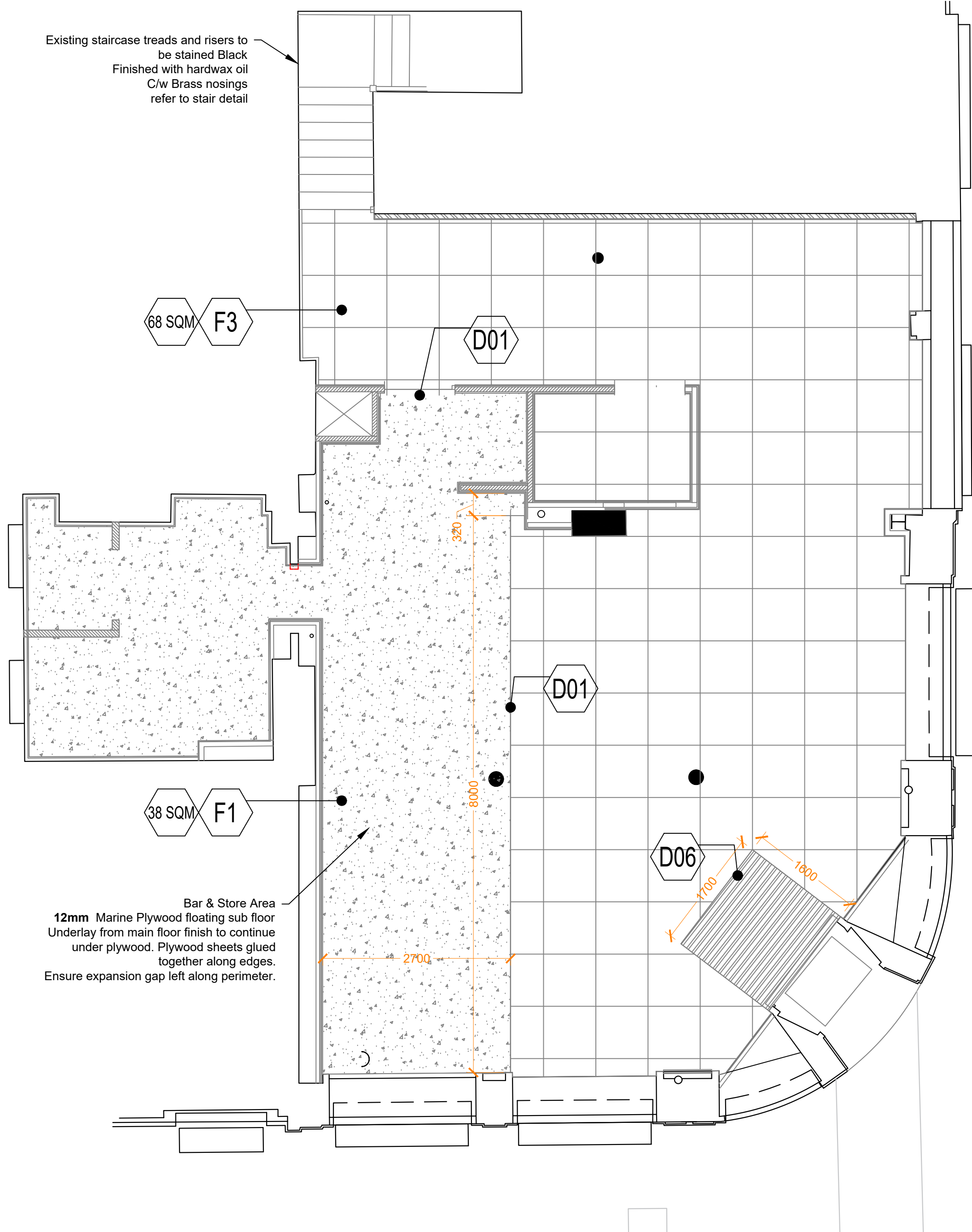
7 Ground Floor | Floor Finishes Layout
