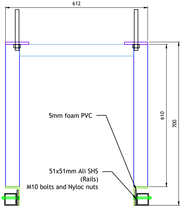
Brackets 4 & 5 Plan view
