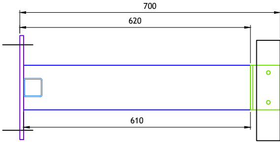
Side view - BKT 1 & 4
