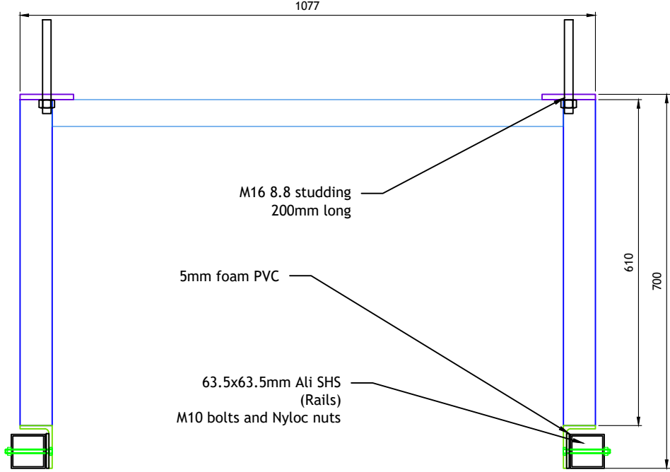
Front Elevations
