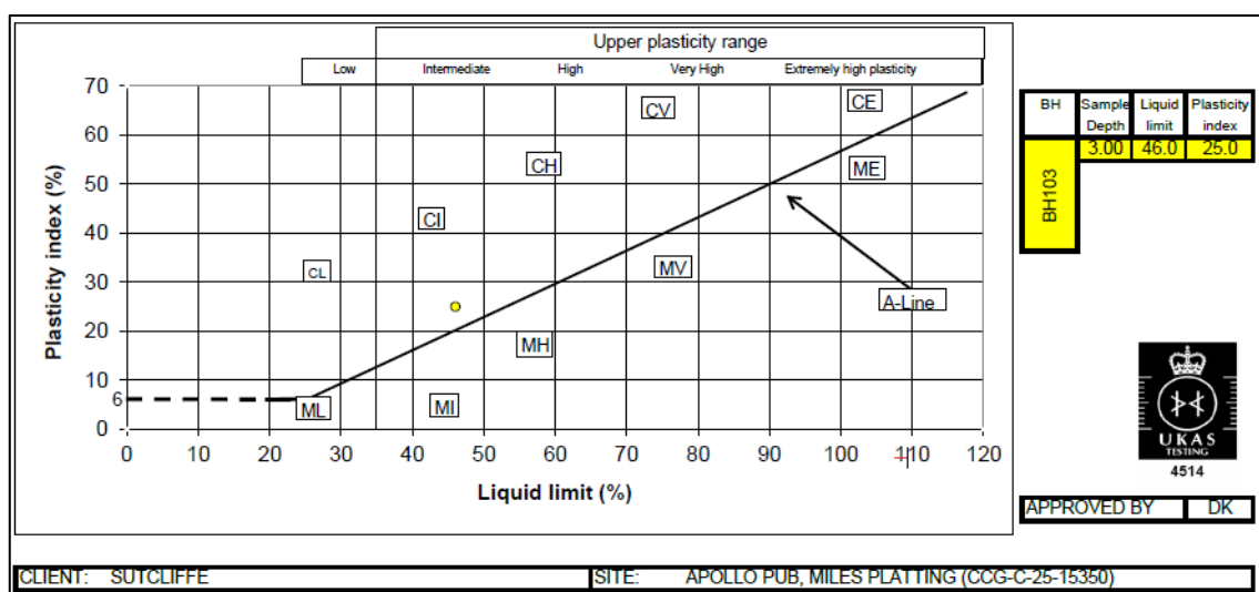
Figure 8: Plasticity Test Results
