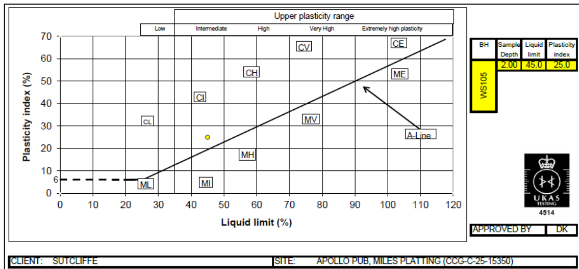
Figure 6: Plasticity Test Results
