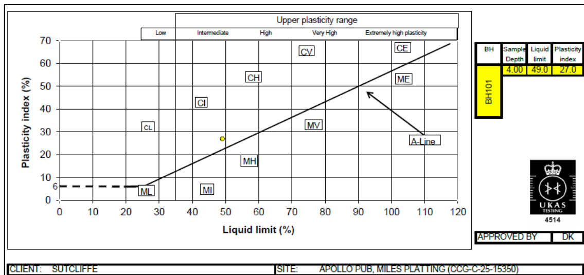
Figure 7: Plasticity Test Results
