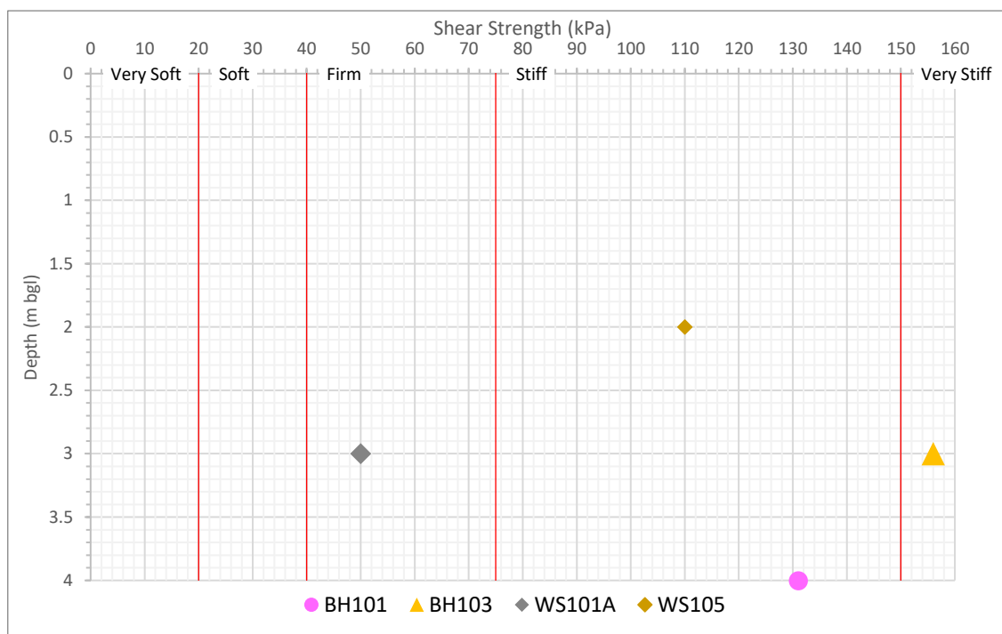
Figure 9: Shear Strength Test Results
