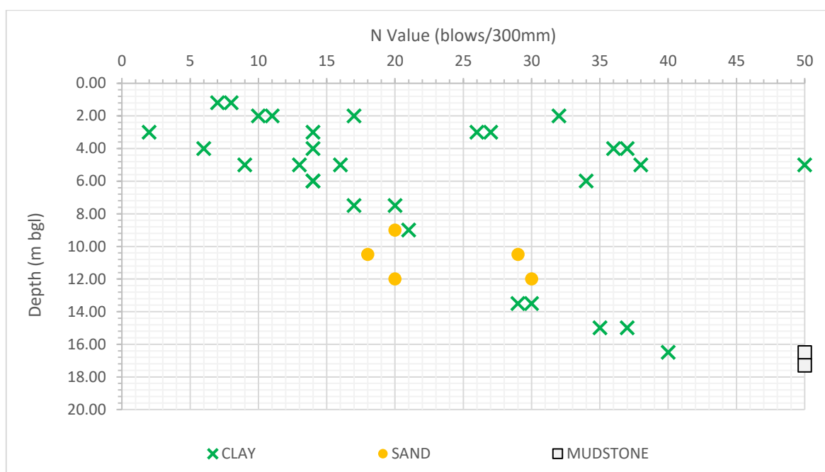
Figure 4: SPT Results
