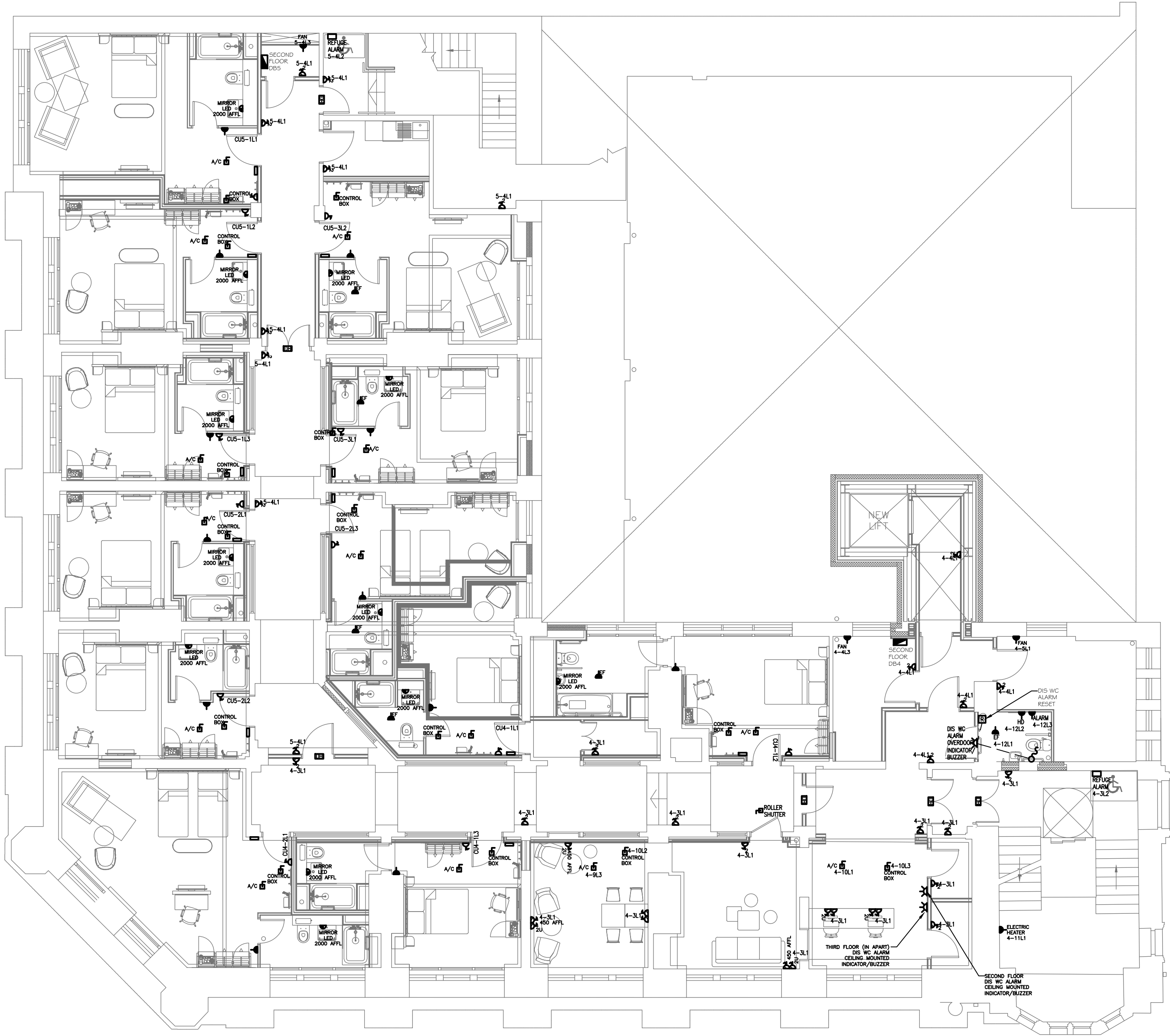
SECOND FLOOR
