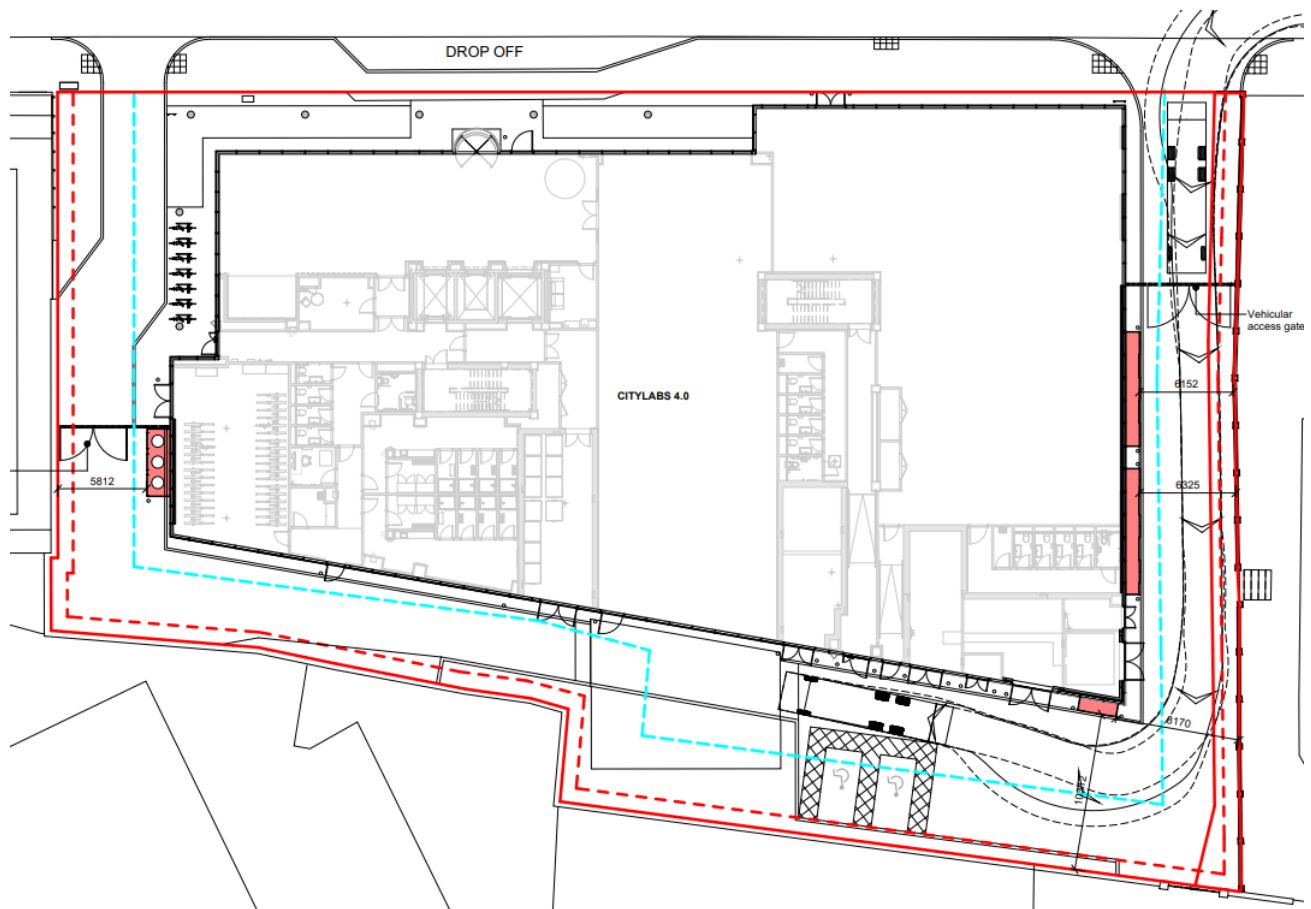
Proposed site plan (gas store location block highlighted in red)
