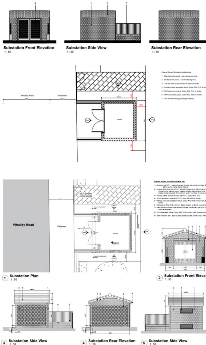
Figure 1 (repeated). Top image previously approved substation, bottom image proposed substation
