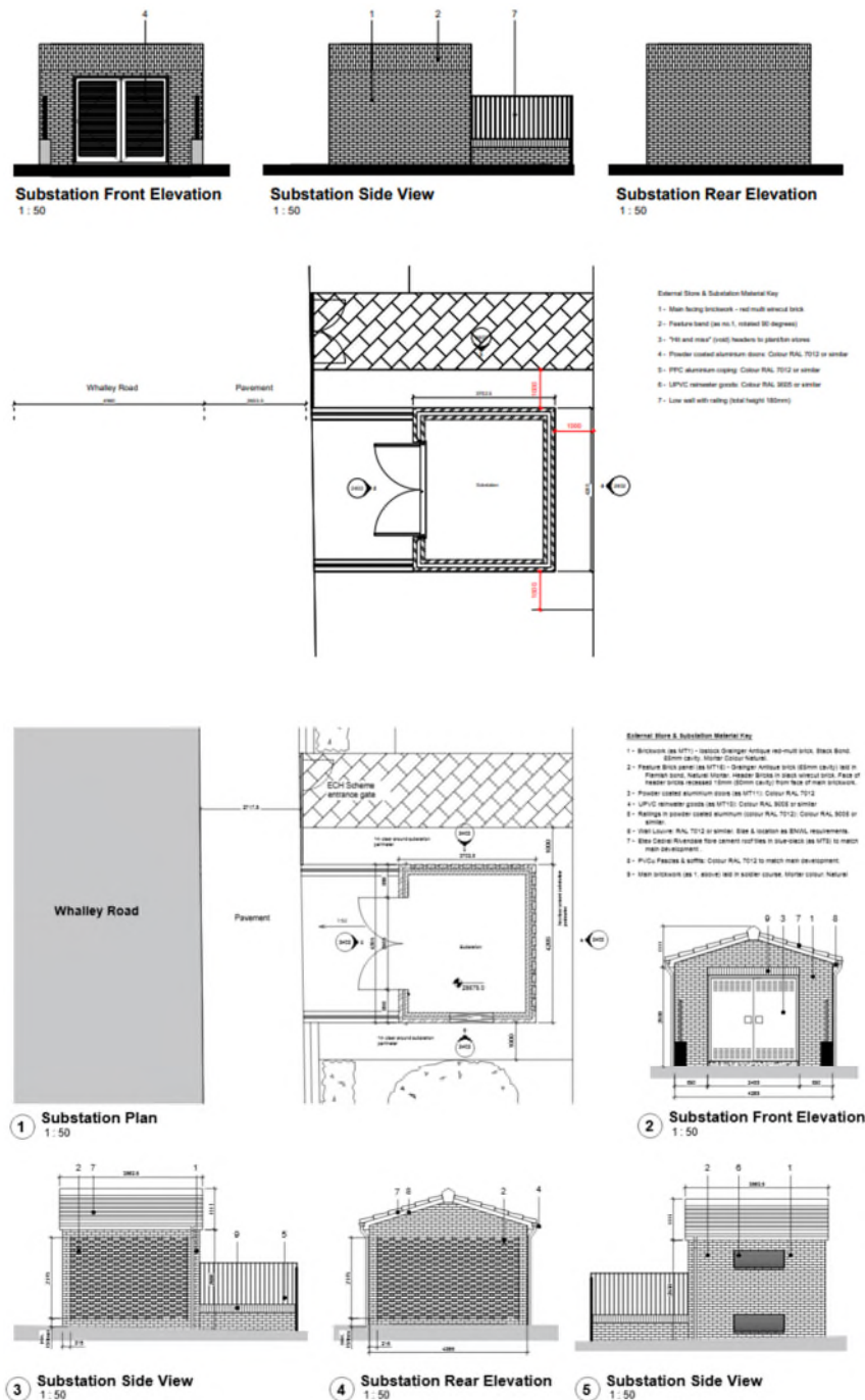
Figure 1. Top image previously approved substation, bottom image proposed substation
