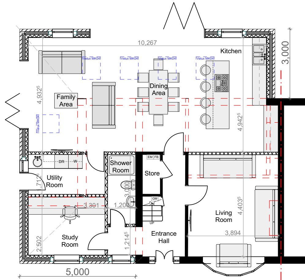
PROPOSED GA GROUND FLOOR PLAN
