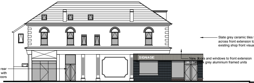
03 PROPOSED SIDE ELEVATION (MONTGOMERY ROAD) Scale 1:100 @ A1
