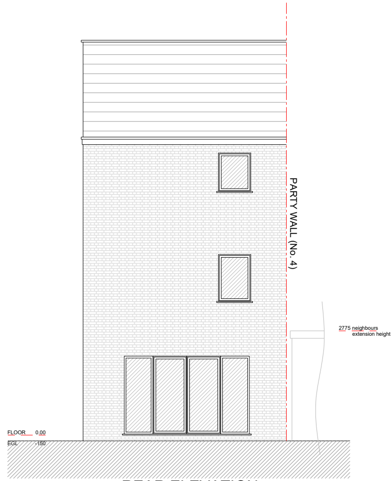
REAR ELEVATION
