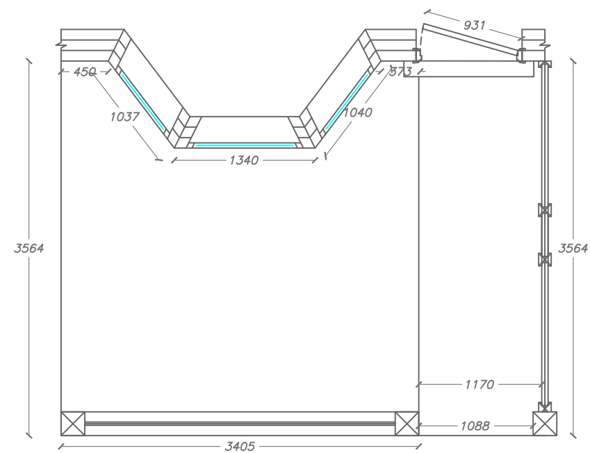
Existing Layout
