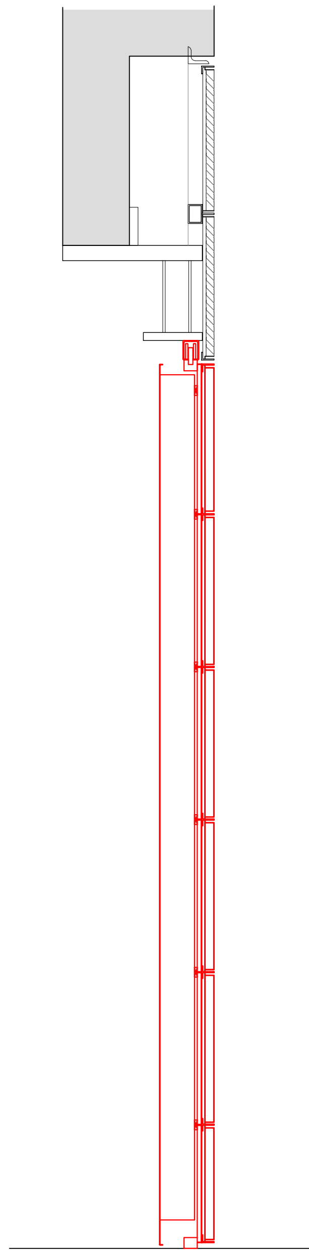
Loading Bay Doors Section A-A, as Existing 1:20
