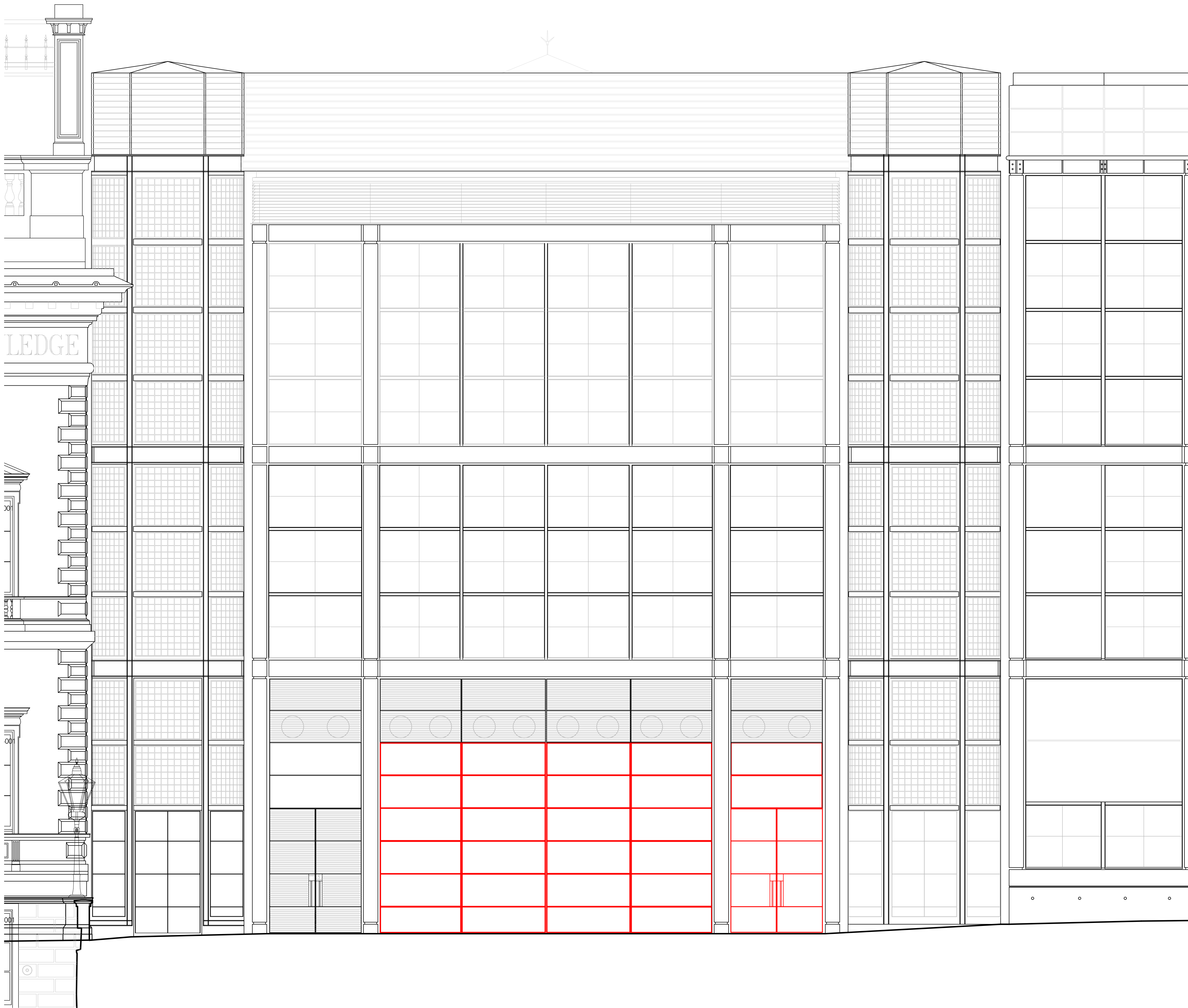
George Street, Elevation as Existing 1:50
