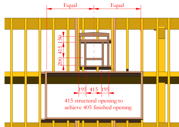
Elevation showing timber framing
