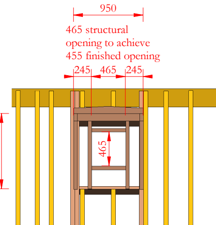
Elevation showing timber framing
