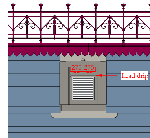
Elevation showing lead covering
