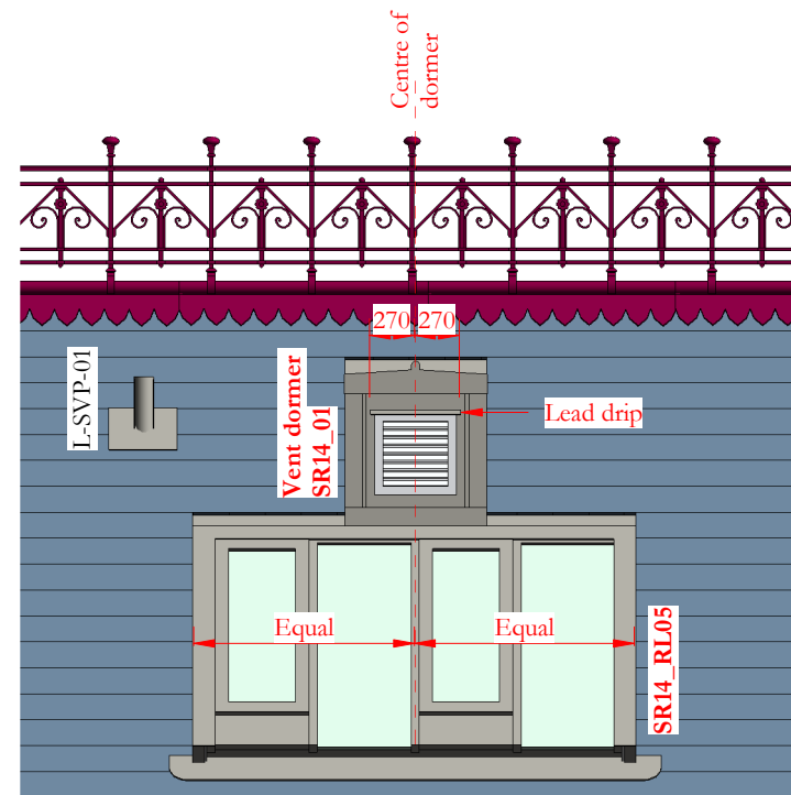
Elevation showing lead covering
