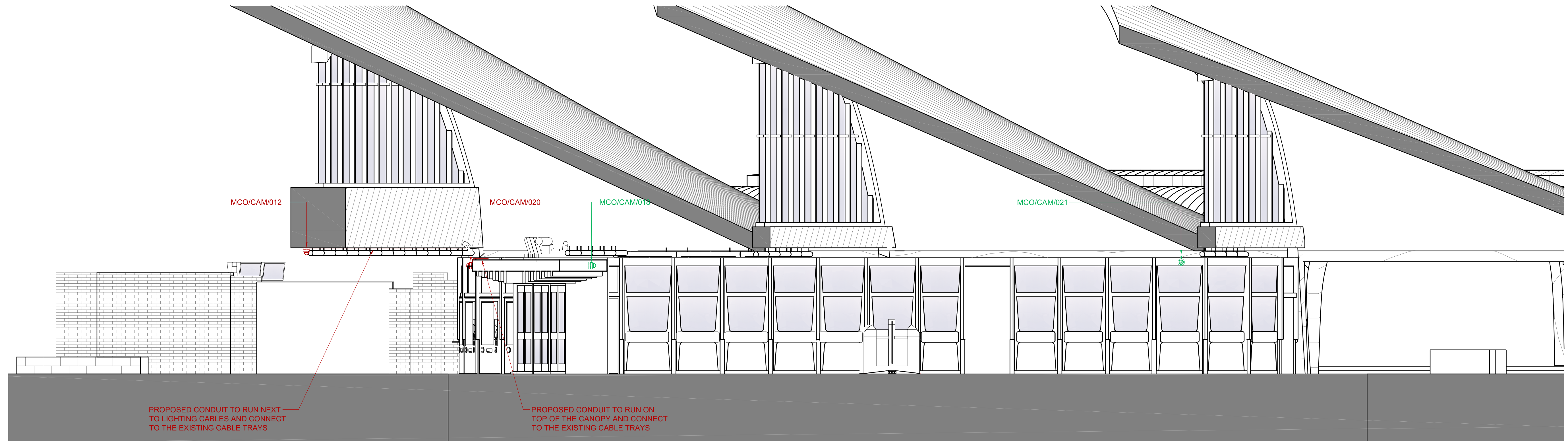
2 SECTION B-B 30 1:50
