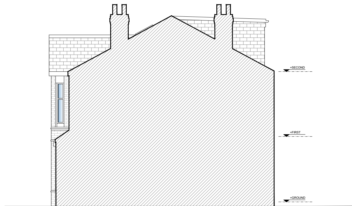
• Existing Side Elevation (From No 127)
