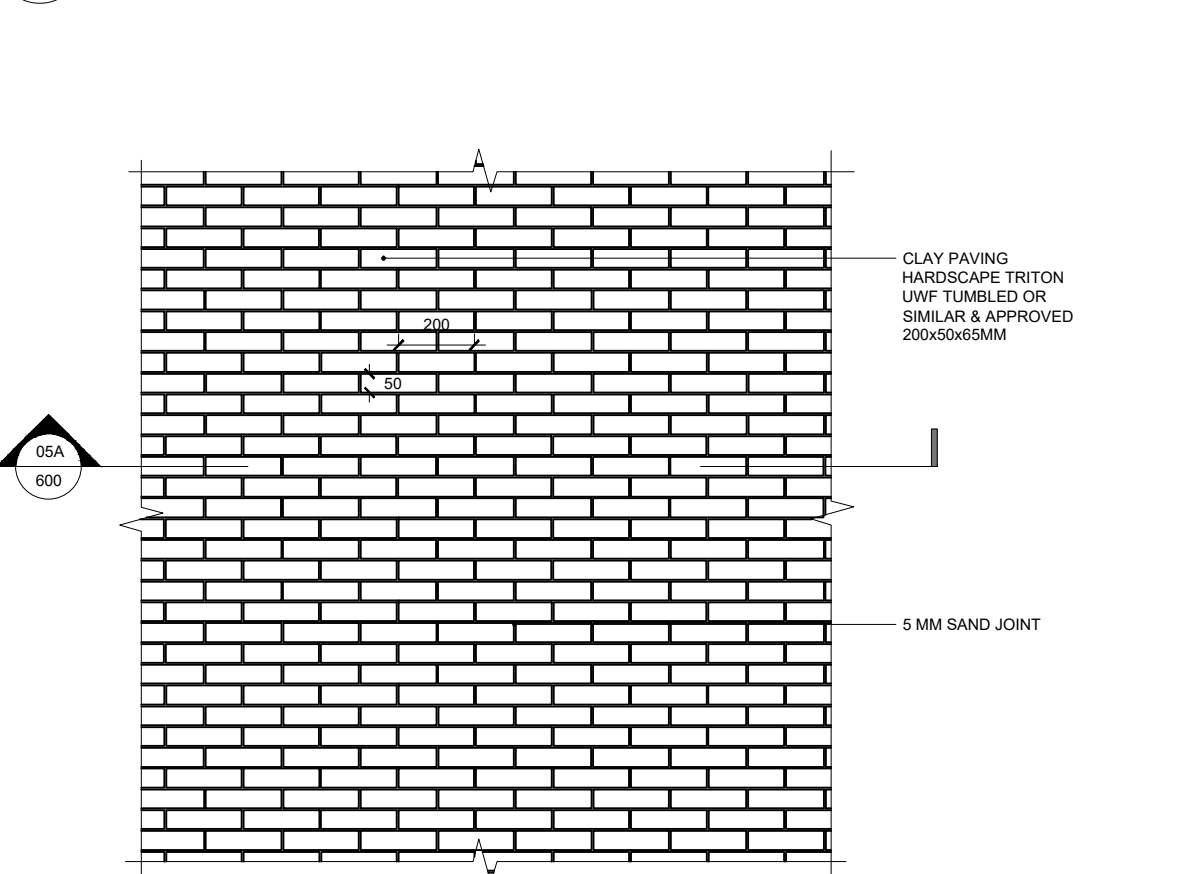
05B 600 PLAN ST05 - CLAY PAVING
