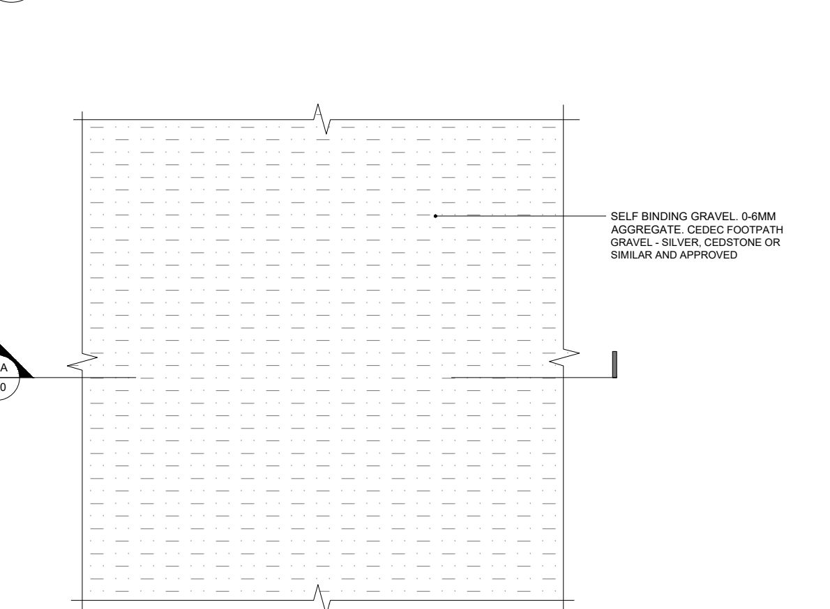
07B 600 PLAN ST07 - SURFACE TYPE 7: SELF BINDING GRAVEL
