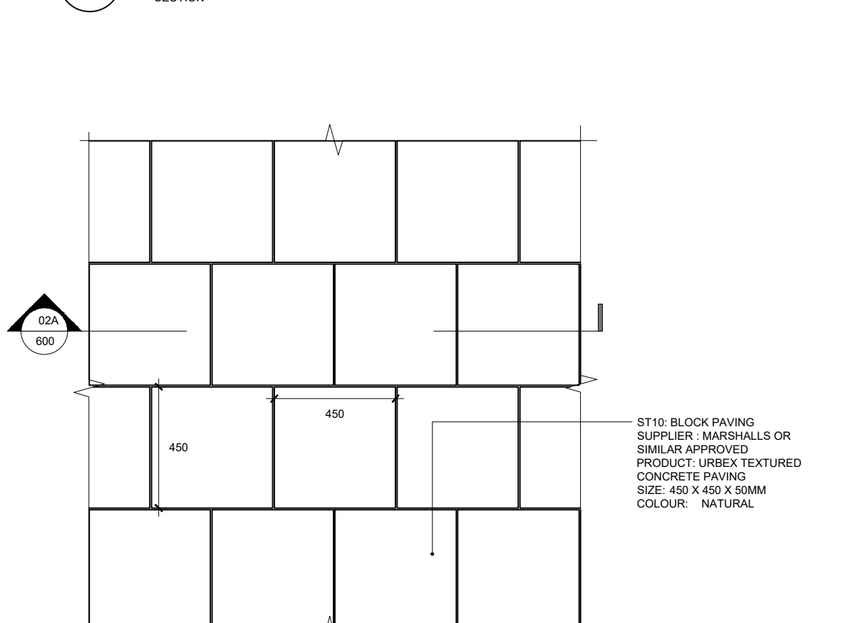
07B 600 PLAN ST10 - CONCRETE PAVING
