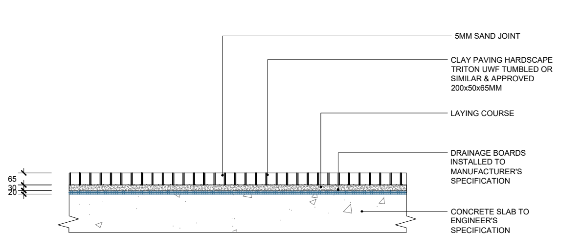
02B 600 PLAN ST02 - CLAY PAVING
