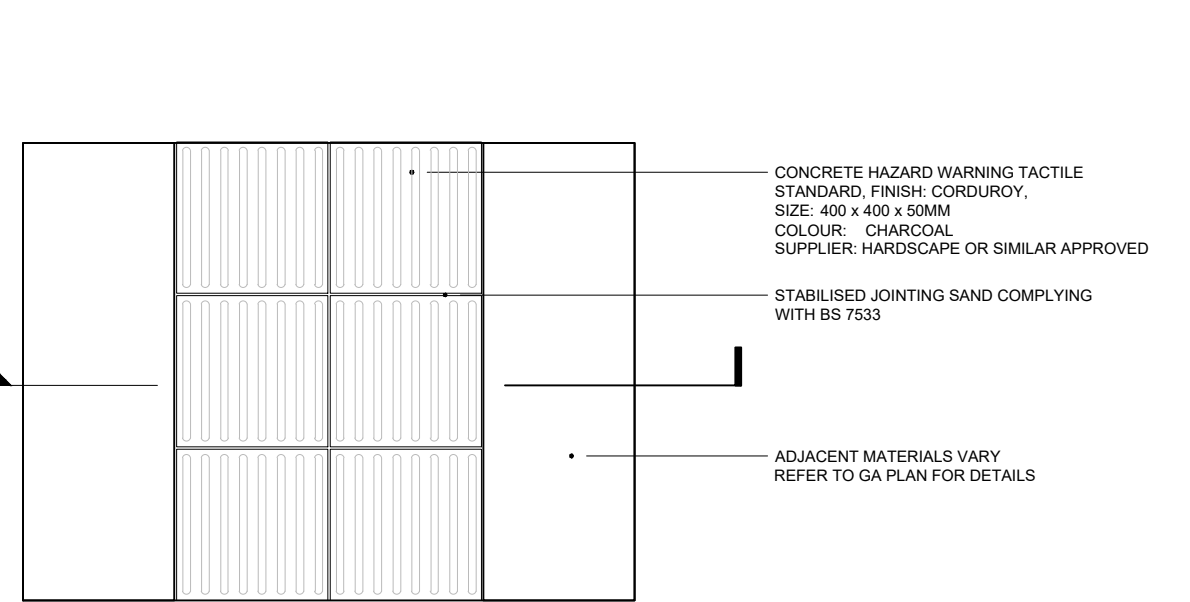
07B 600 PLAN SURFACE TYPE 8: TACTILE PAVING
