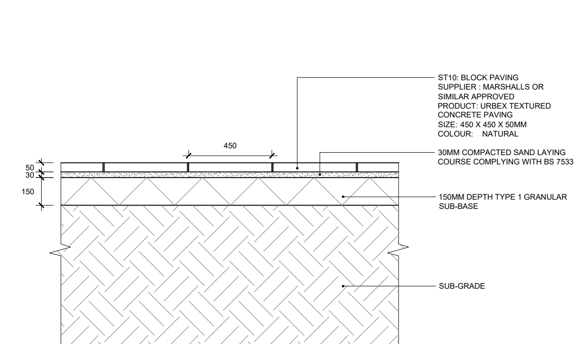
07A 600 SECTION ST10 - CONCRETE PAVING
