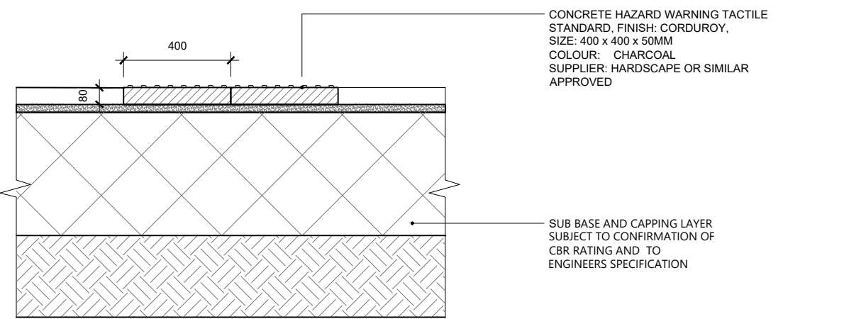
07A 600 SECTION SURFACE TYPE 8: TACTILE PAVING
