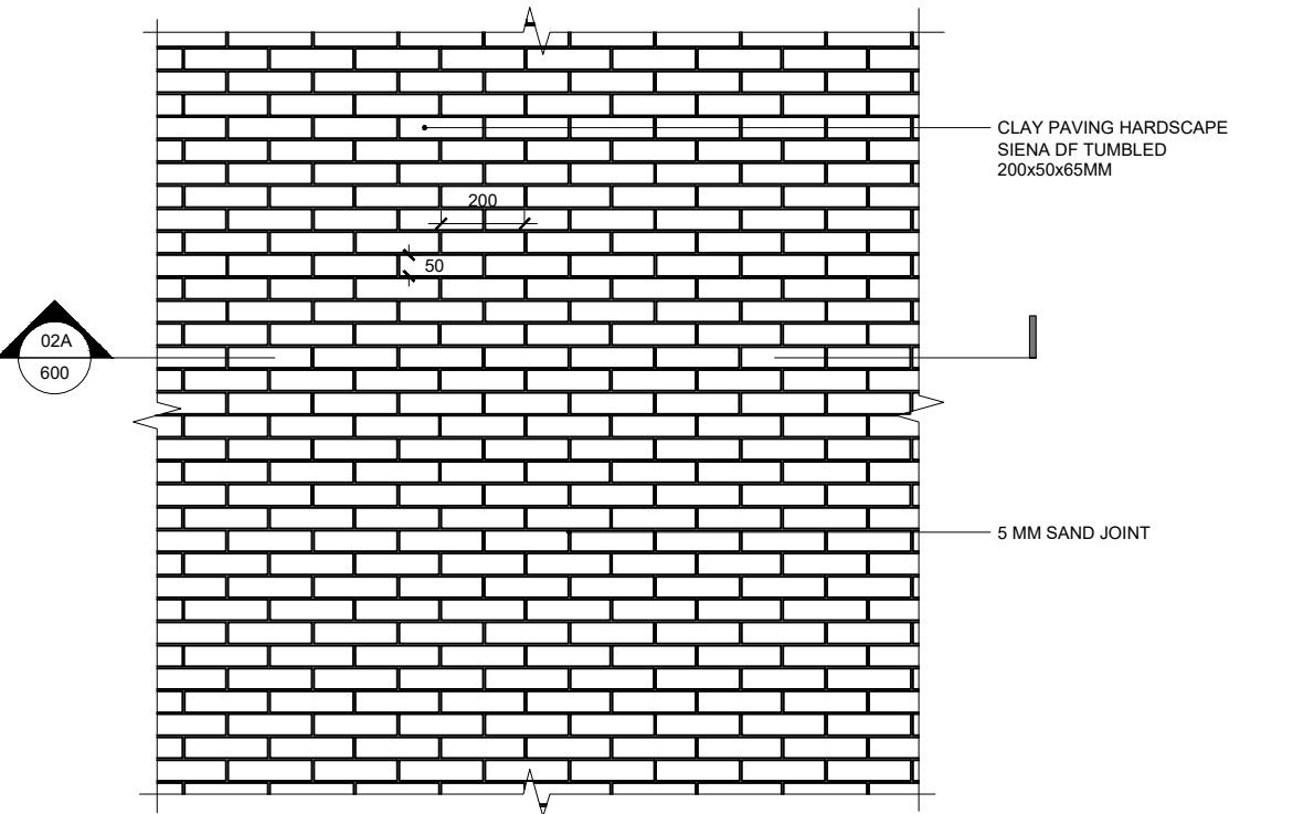
02B 600 PLAN ST02 - CLAY PAVING
