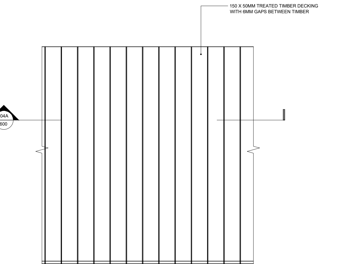
04B 600 PLAN ST04 - COMPOSITE DECKING
