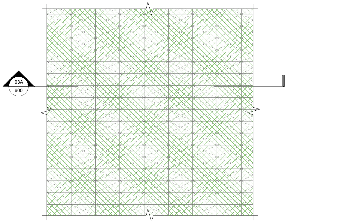
03B 600 PLAN ST03 - GREEN BRICK
