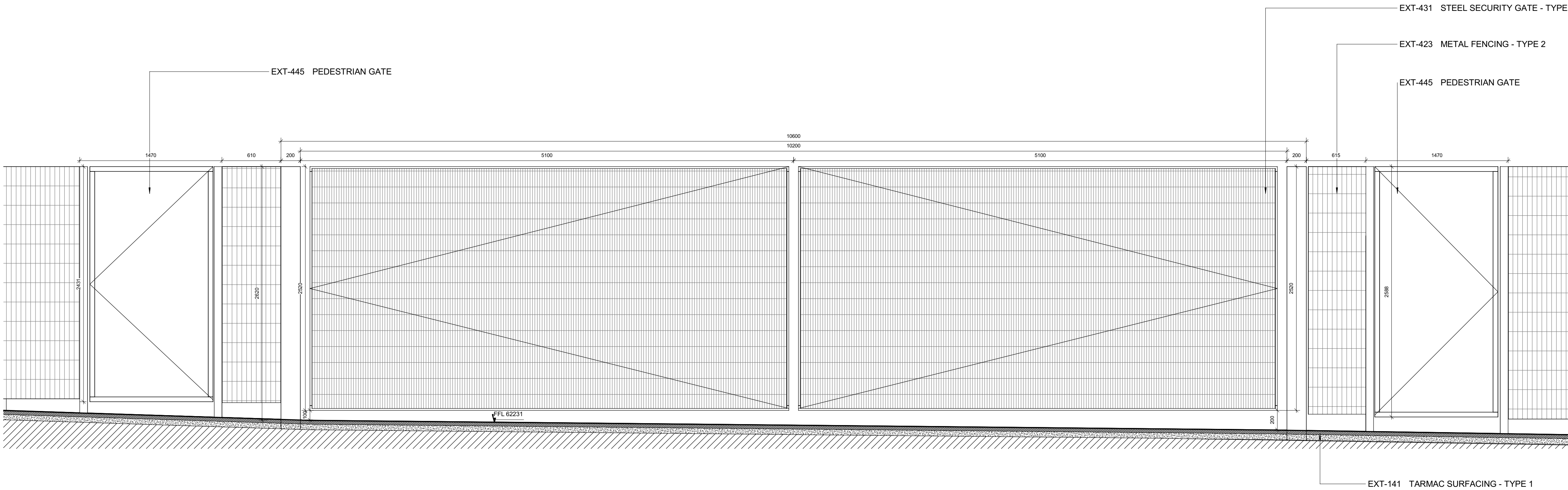
1 STEEL SECURITY GATE AND FENCE ELEVATION
