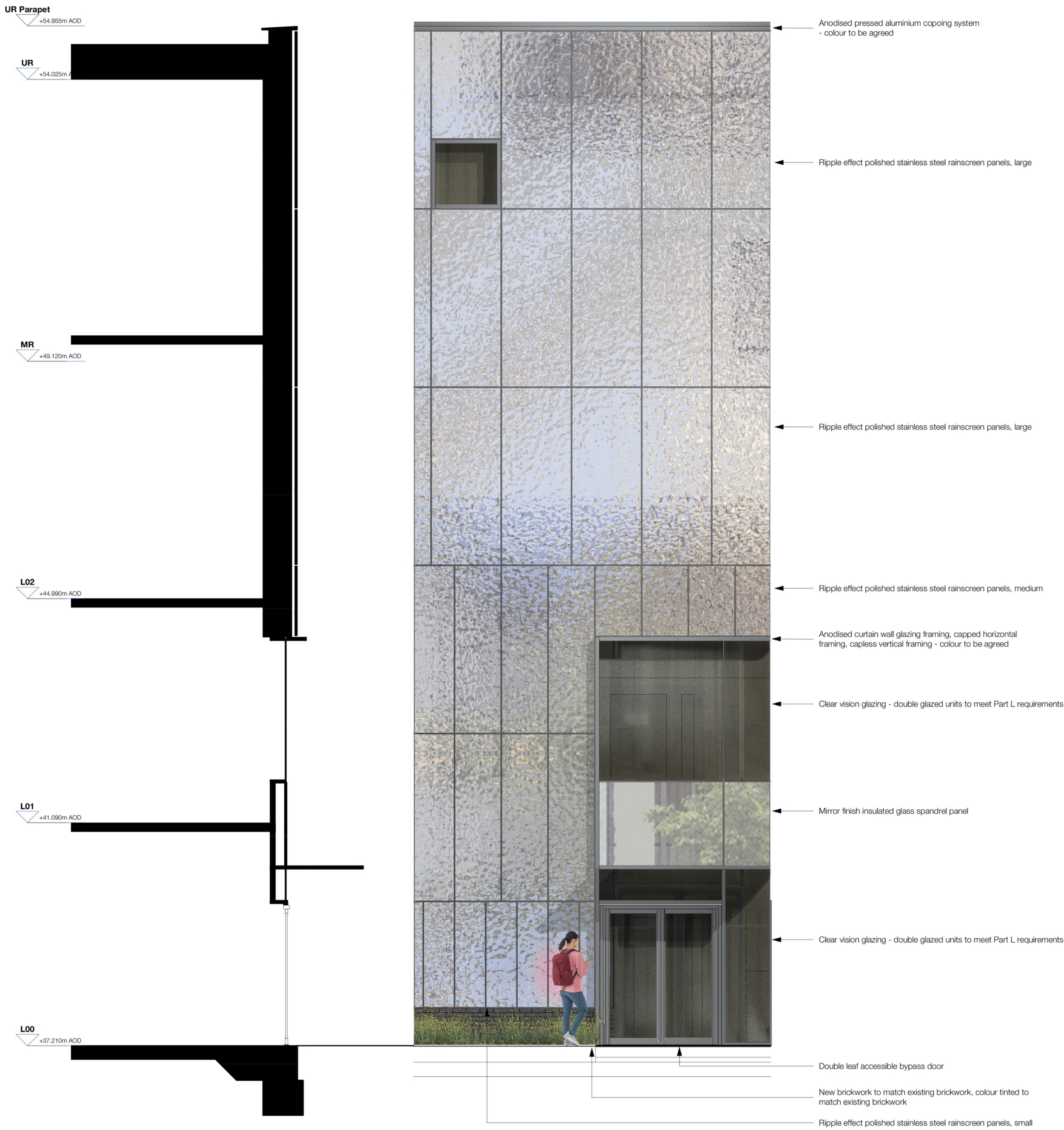
2 Proposed - Bay Study C Section 1 : 50
