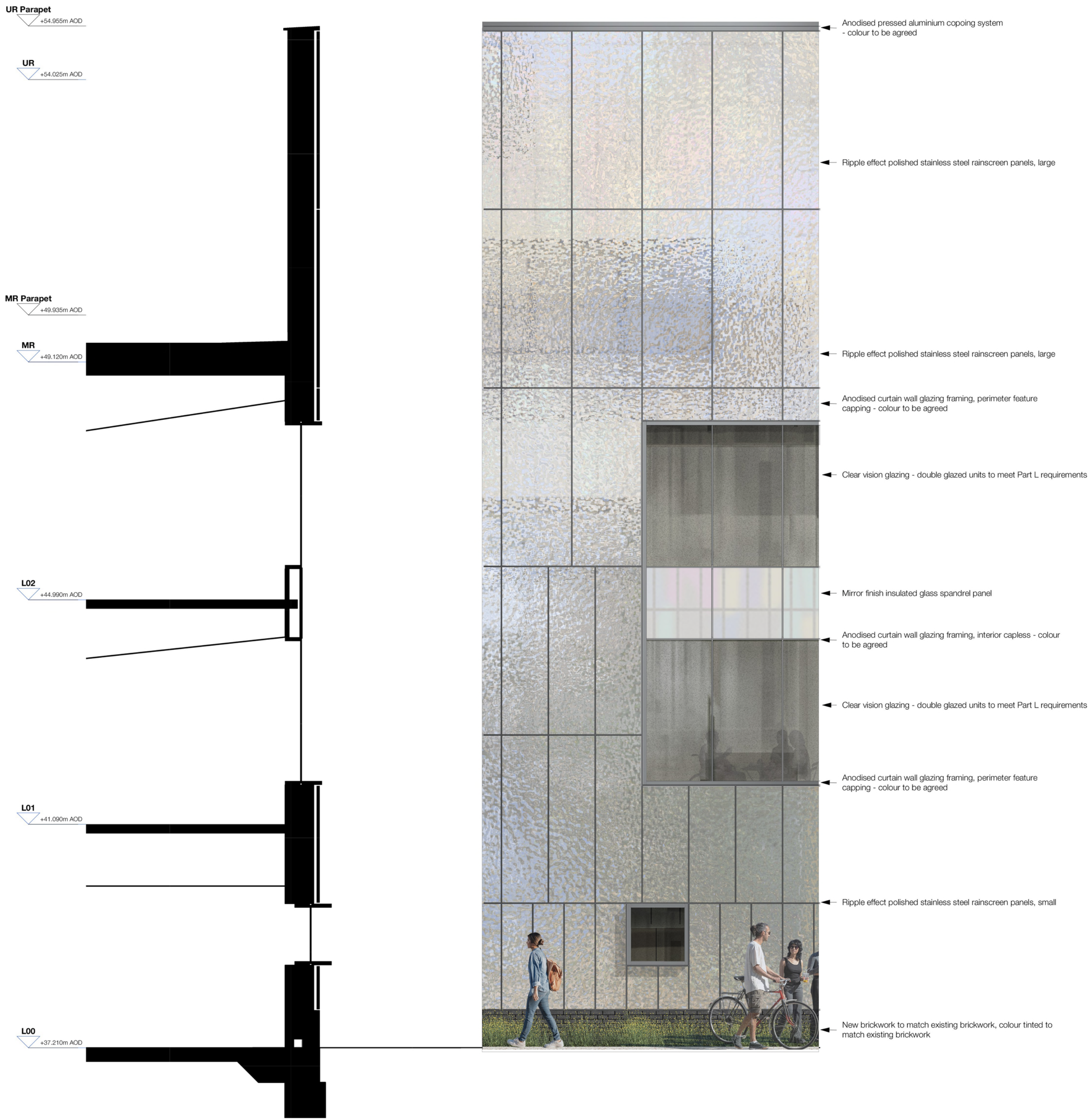
1 Proposed - Bay Study D Section 1 : 50
