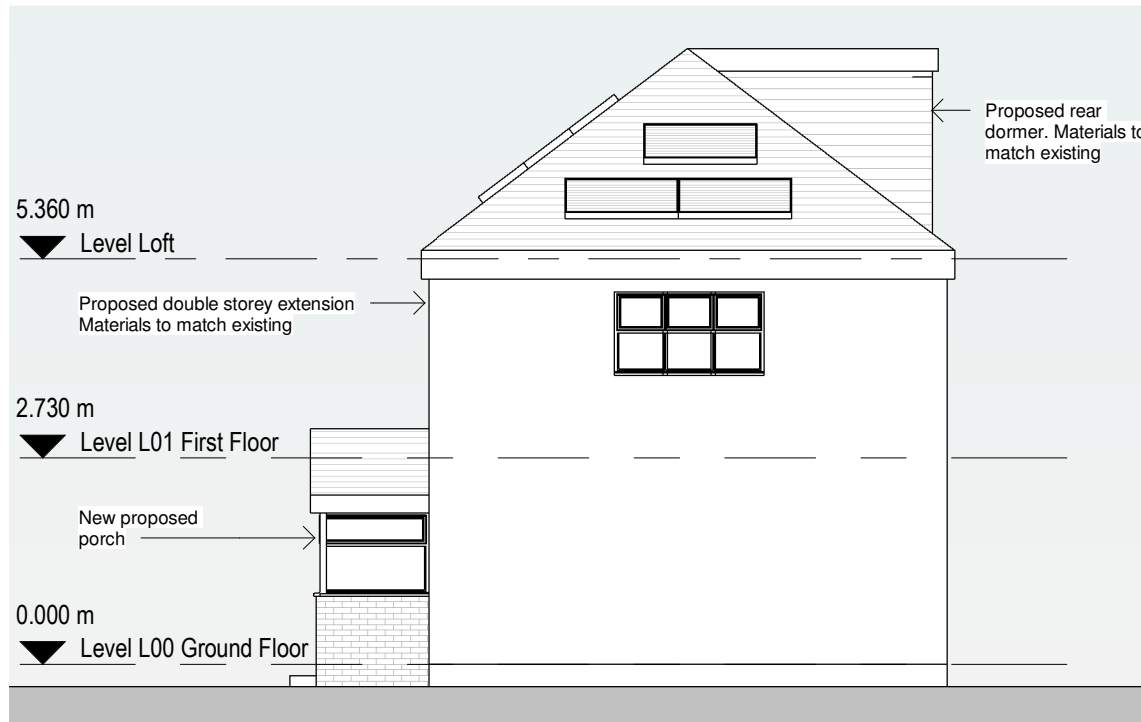
2 Proposed East Elevation 1 : 100
