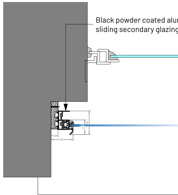
1 Window A Reveal Plan - Secondary Glazing Scale: 1:5
