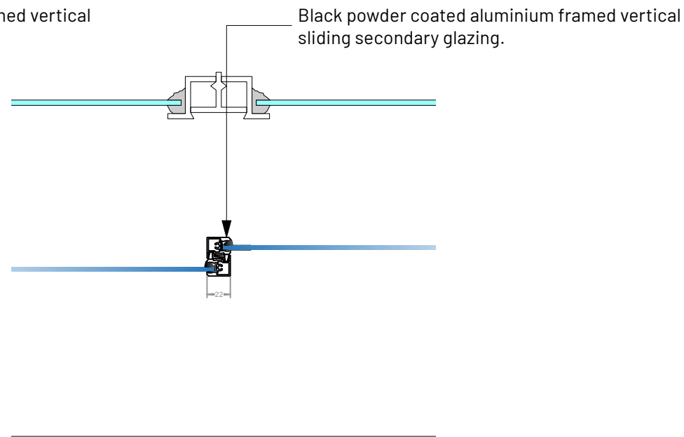
2 Window A Junction Plan Between Frames Scale: 1:5
