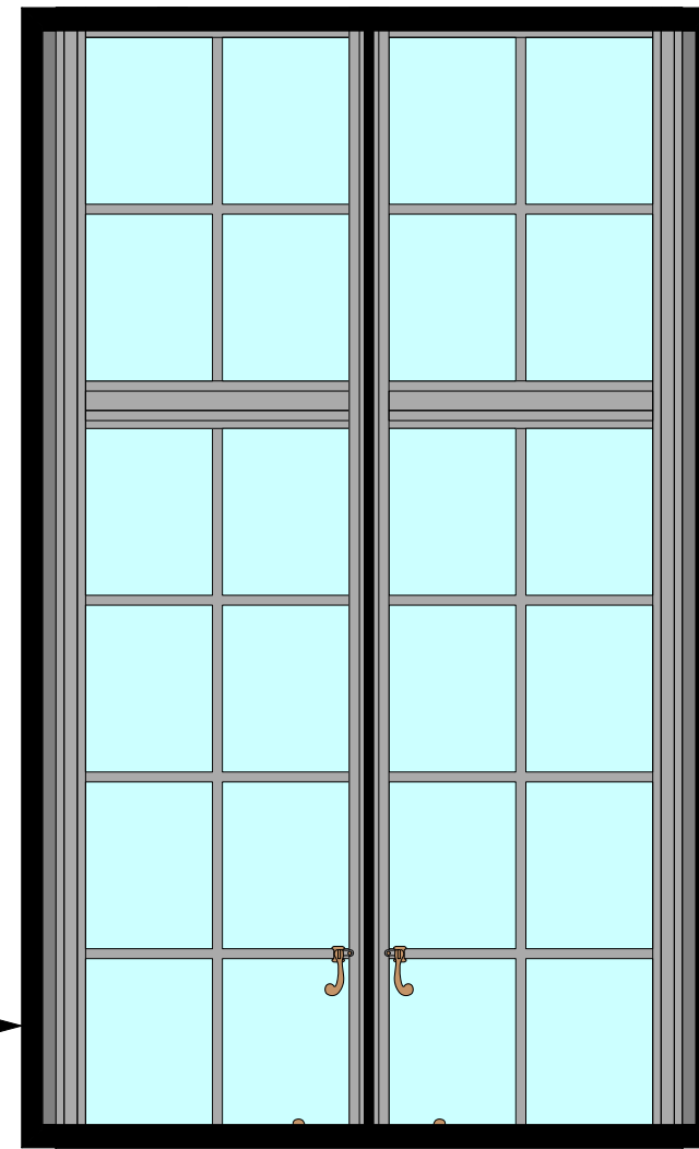
4 Window A Type 1 Internal Elevation Scale: 1:20
