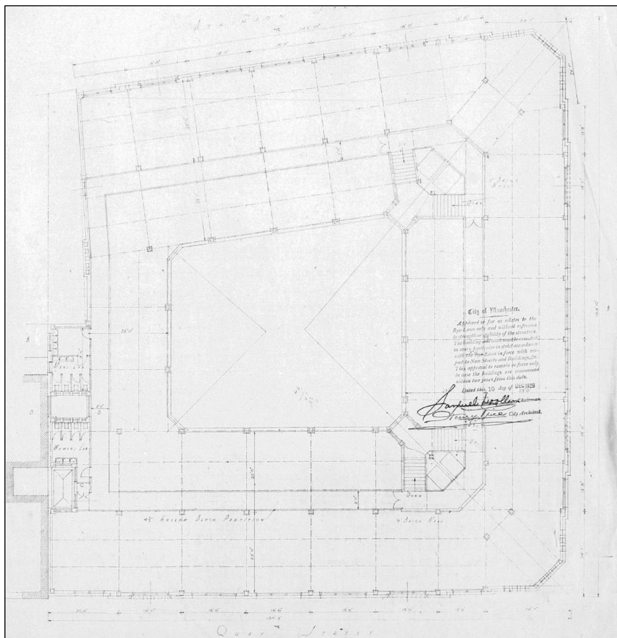
Image F: First floor plan (1929)
