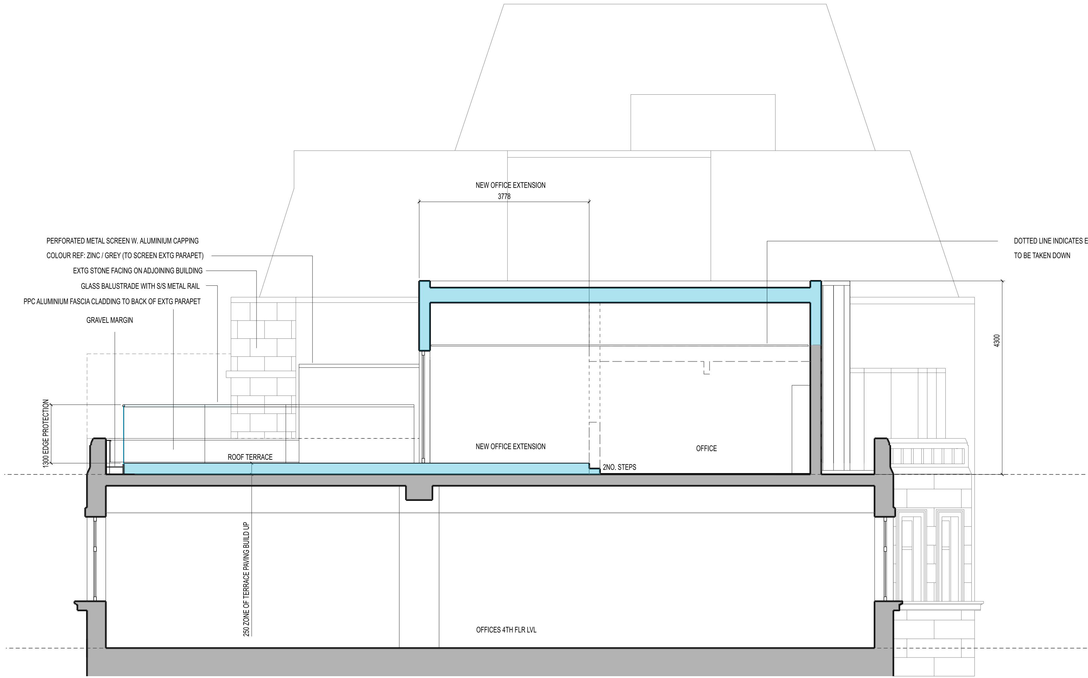
PROPOSED CROSS-SECTION AA
