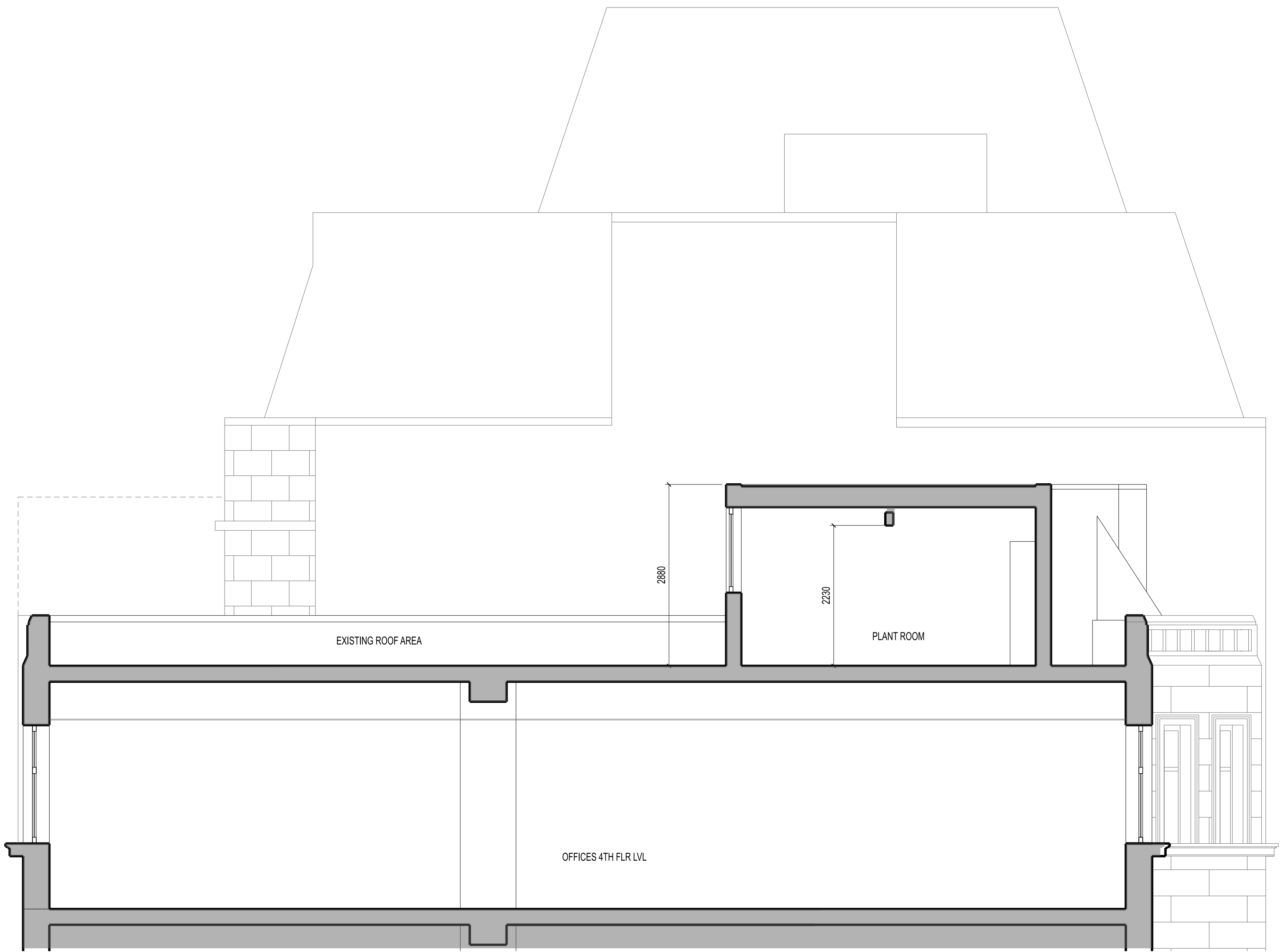
EXISTING CROSS-SECTION AA
