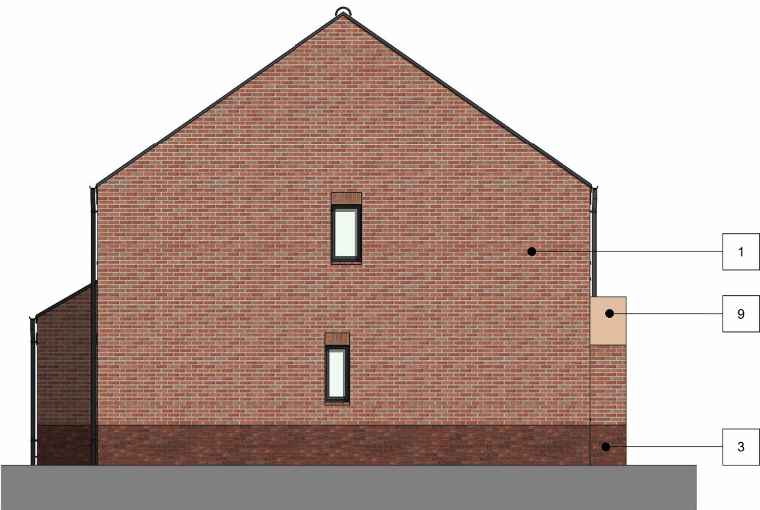
Left Elevation 1 : 100
