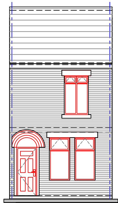
EXISTING FRONT ELEVATION 1:100
