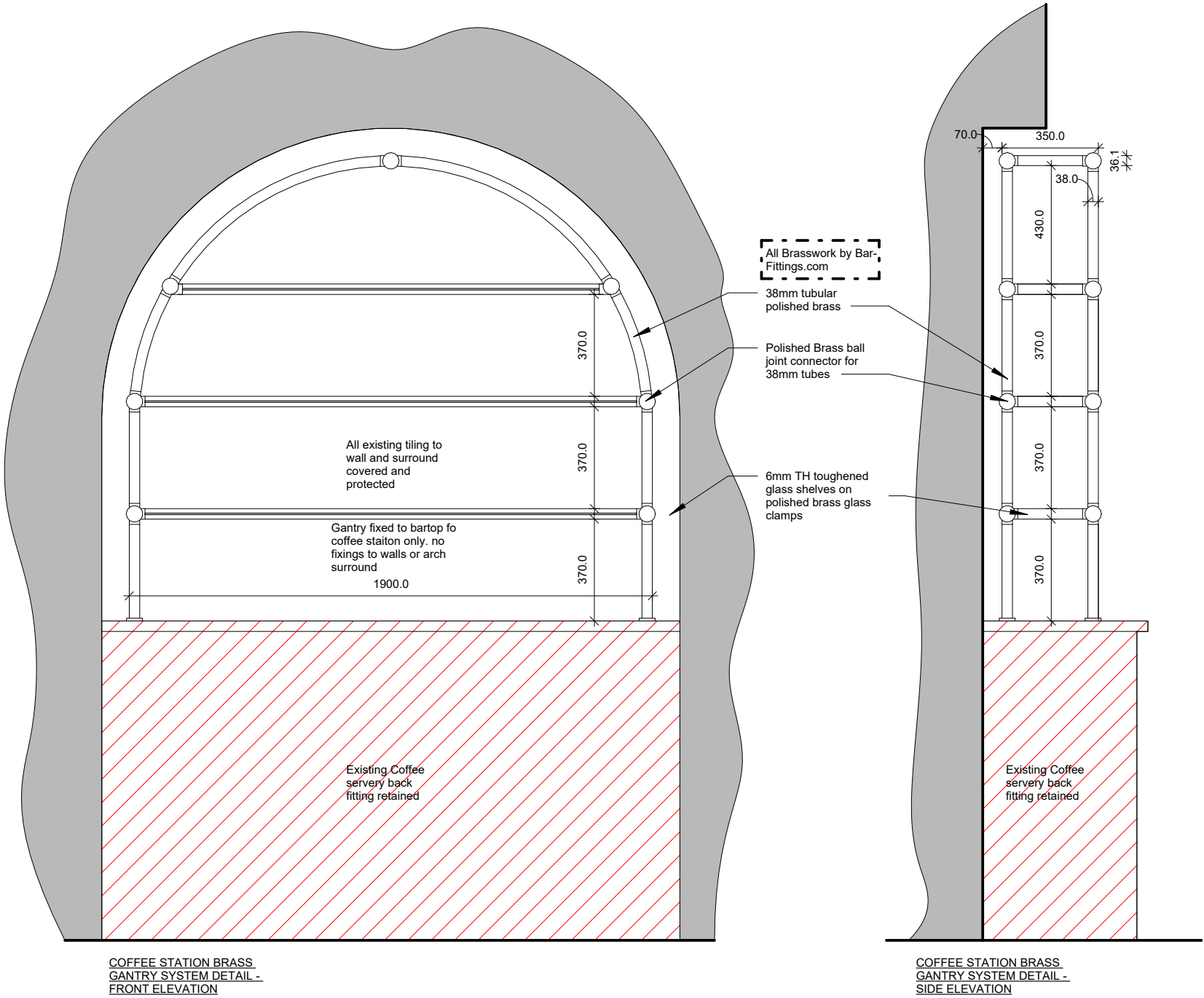
Coffee Station Brass Gantry 1 : 20
