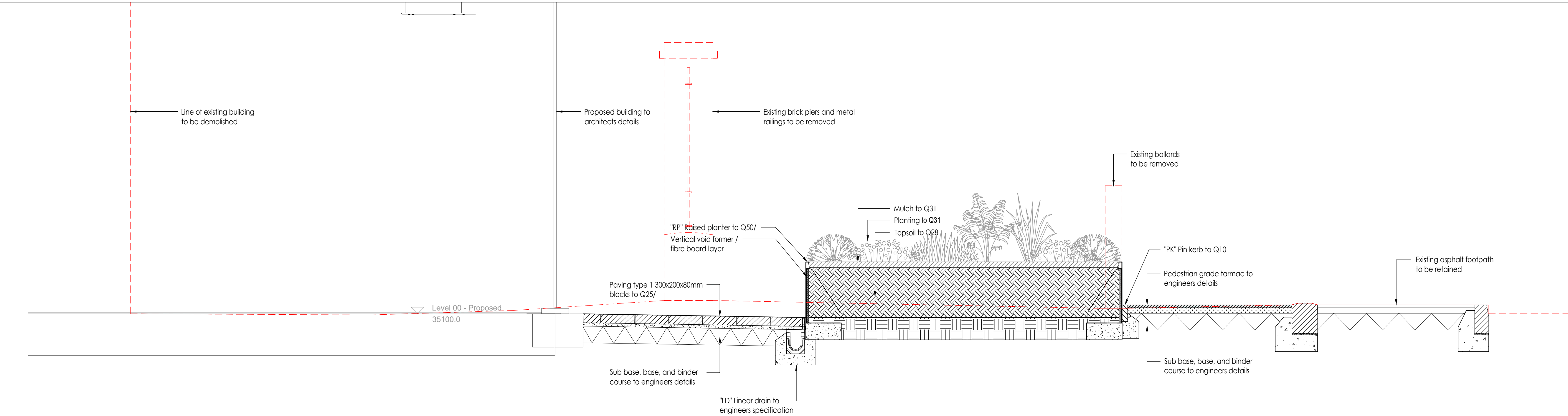
Section 6 Scale 1:20
