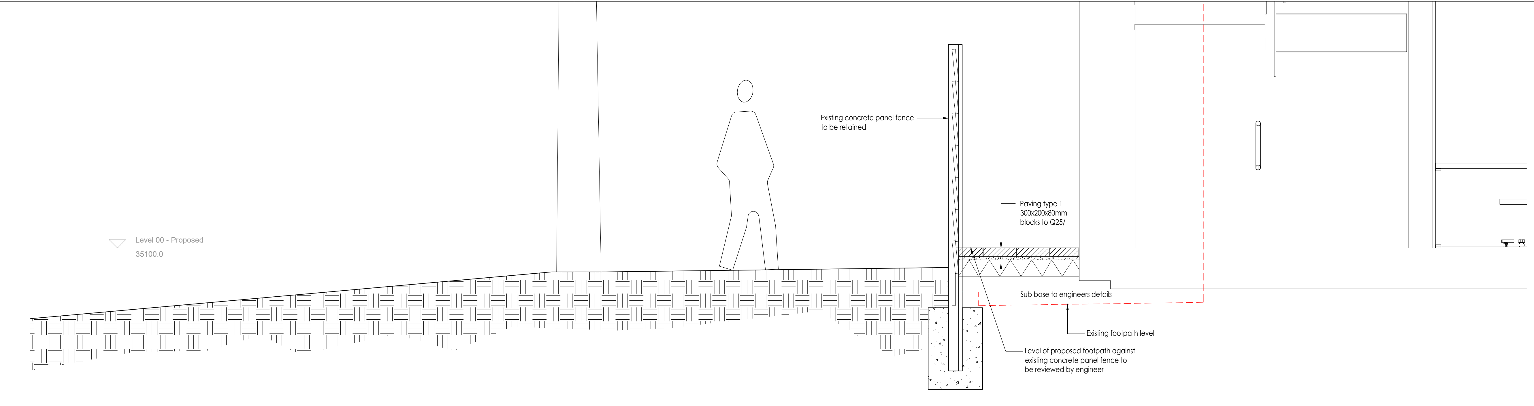
Section 5 Scale 1:20
