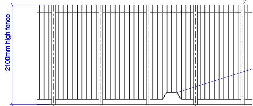
typical fence: proposed elevation
