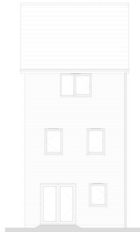
Rear Elevation
