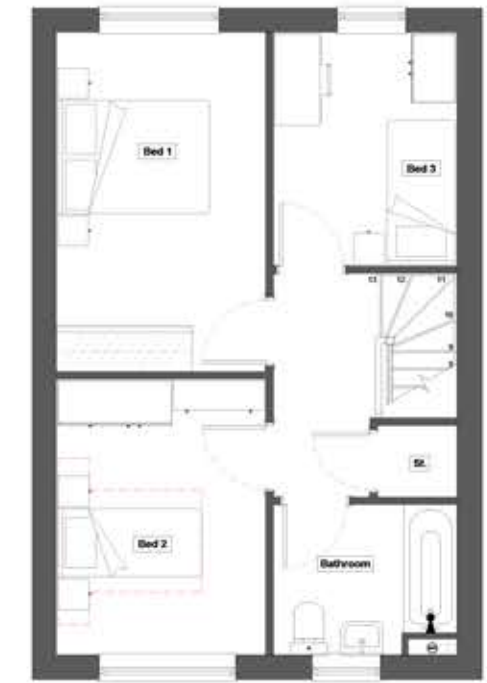
First Floor Scale - 1:100
